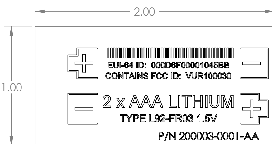
LABEL MATERIAL: .002" POLYESTER, PEARL WHITE
