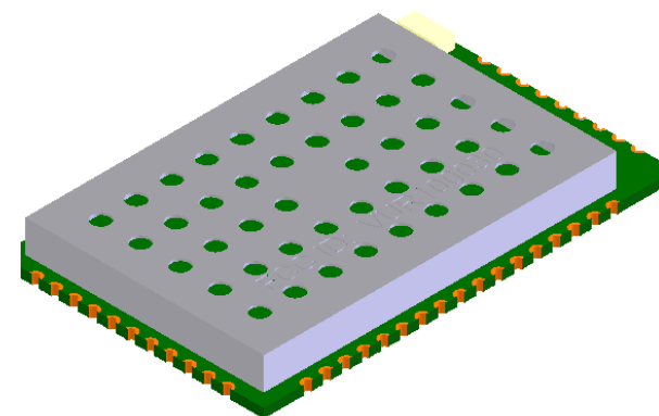
MODULE FCC ID ETCHED ONTO OPTIONAL SHIELD
