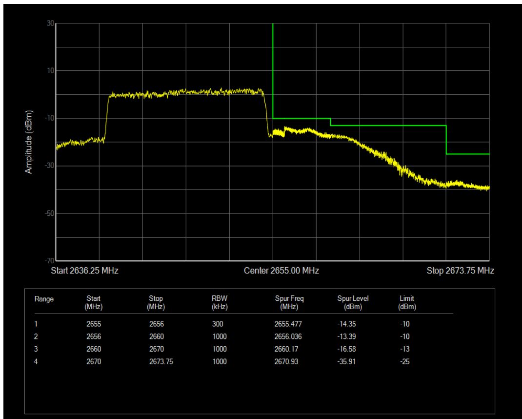
Band41(2545-2655) QAM16 BW=15MHz Channel=41165 RB Size=75 Position=#0
