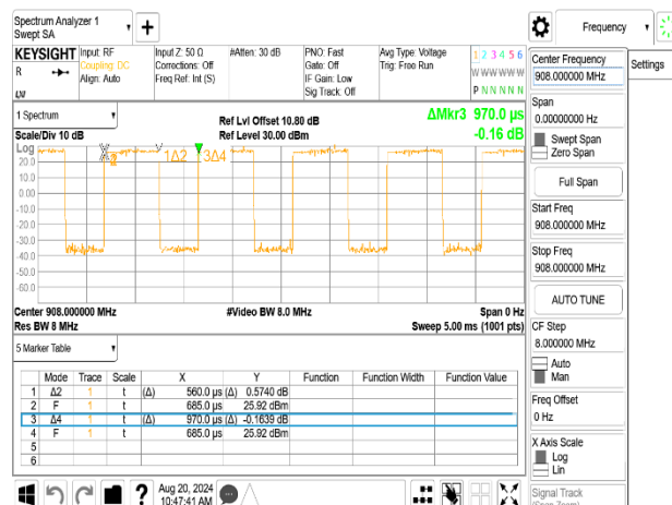
OFDM 8M LowCH-908
