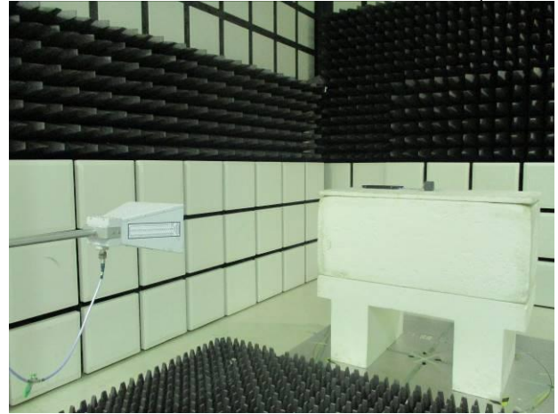
FCC_15_247_902~928MHz_OFDM_Radiated_Setup
