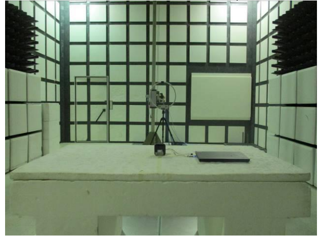
FCC 15 247 BLE Radiated Setup
