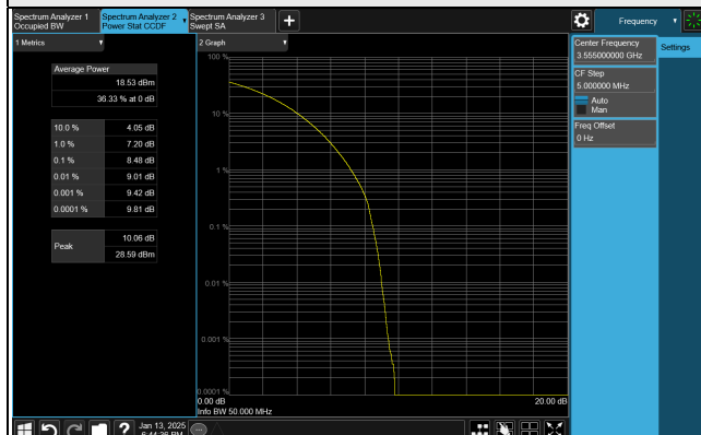
40MHz / Antenna 0 / 16QAM
