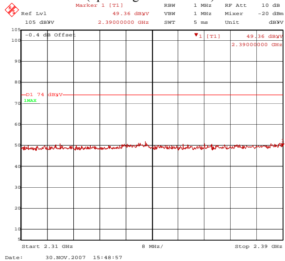
Lowest Channel (operating at 2402 MHz): PEAK
