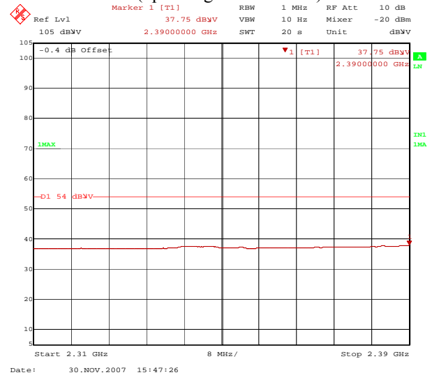
Lowest Channel (operating at 2402 MHz): AVERAGE
