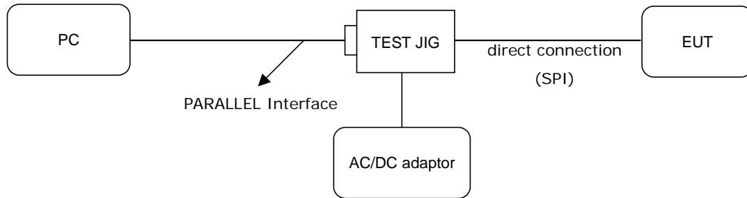
[ System Block Diagram of Test Configuration ]
