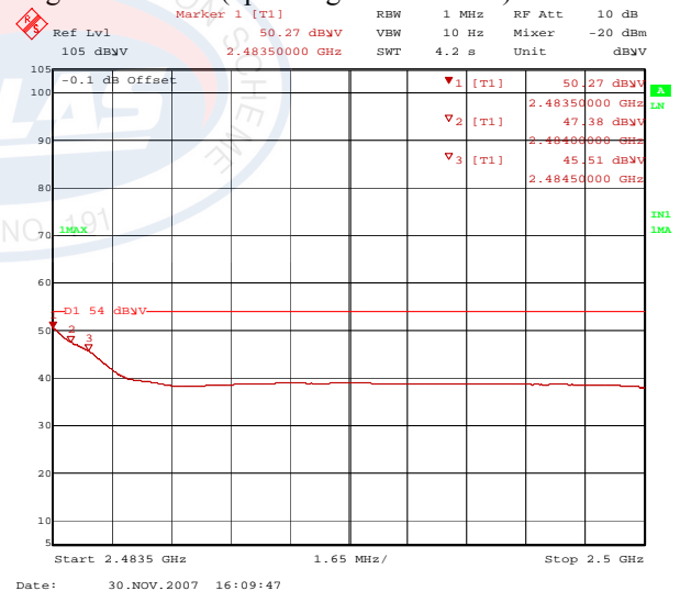
Highest Channel (operating at 2480 MHz): AVERAGE
