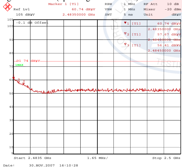
Highest Channel (operating at 2480 MHz): PEAK
