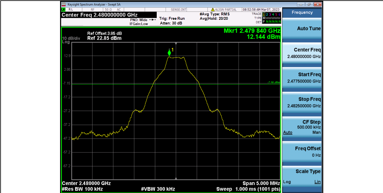
2_Bandedge_NVNT_ANT1_1-DH5_2480
