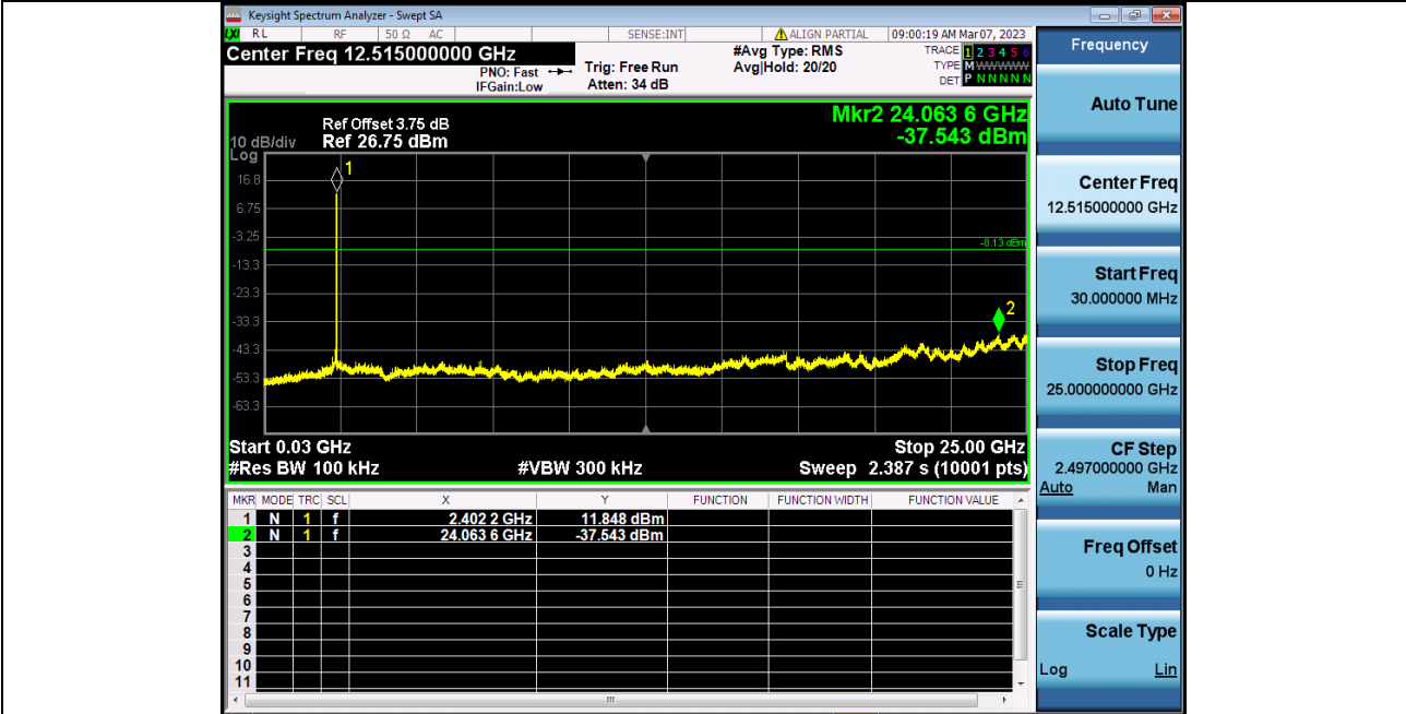
2_Spurious Emissions_NVNT_ANT1_2-DH5_2402
