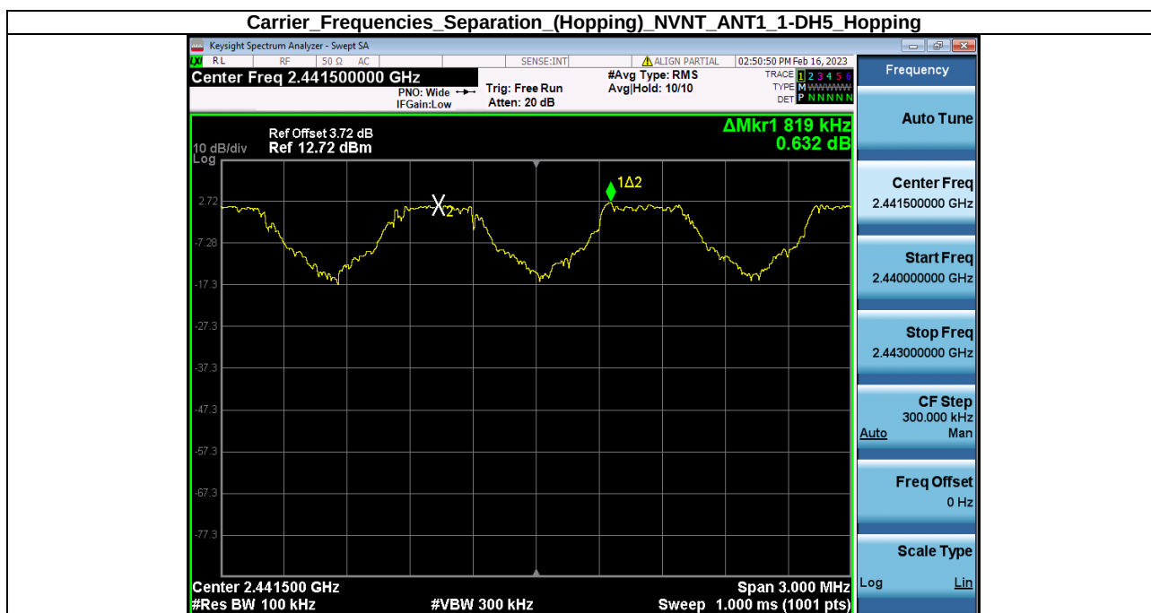
Carrier_Frequencies_Separation_(Hopping)_NVNT_ANT1_1-DH5_Hopping
