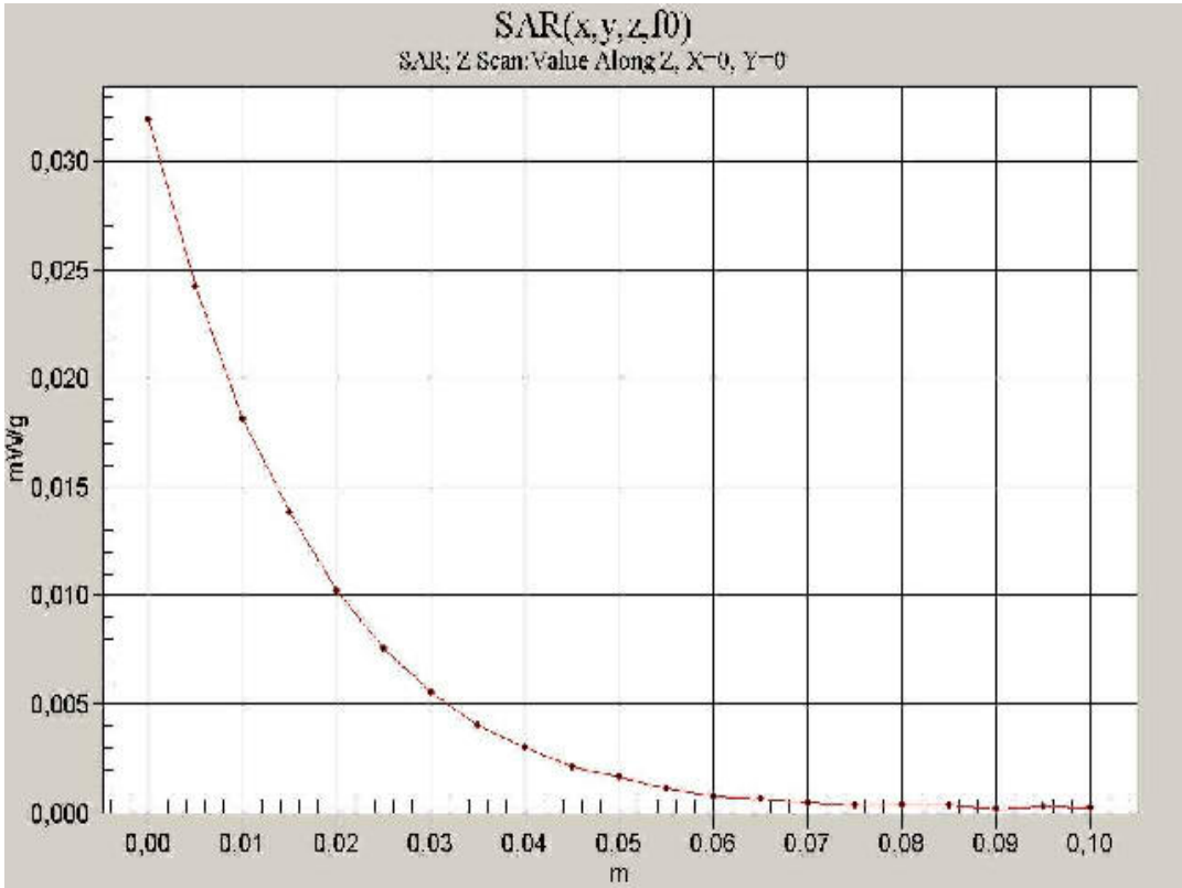
Photo 13: Z-axis scans 1900MHz body
