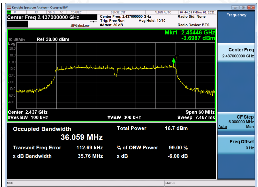
Test_Graph_802.11n40_ANT1_2437_MCS0_DTSBW
