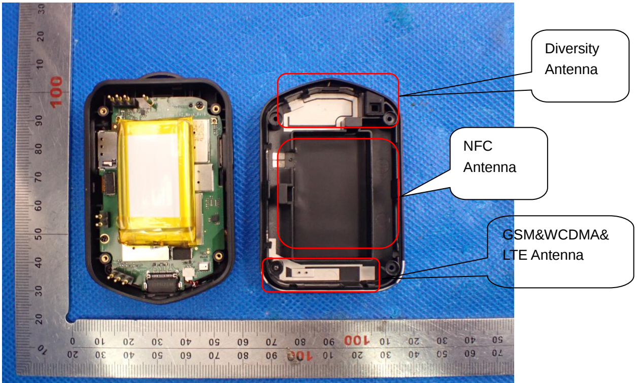
OPEN VIEW OF EUT(FIGURE 2)
