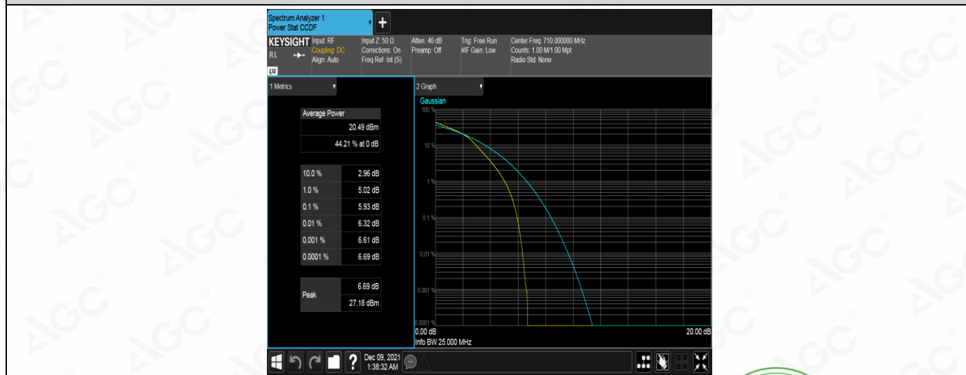
Band17-5MHz-16QAM-23790-25RB#0
