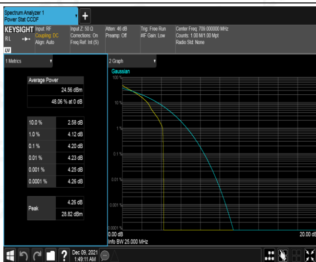
Band17-10MHz-QPSK-23780-50RB#0
