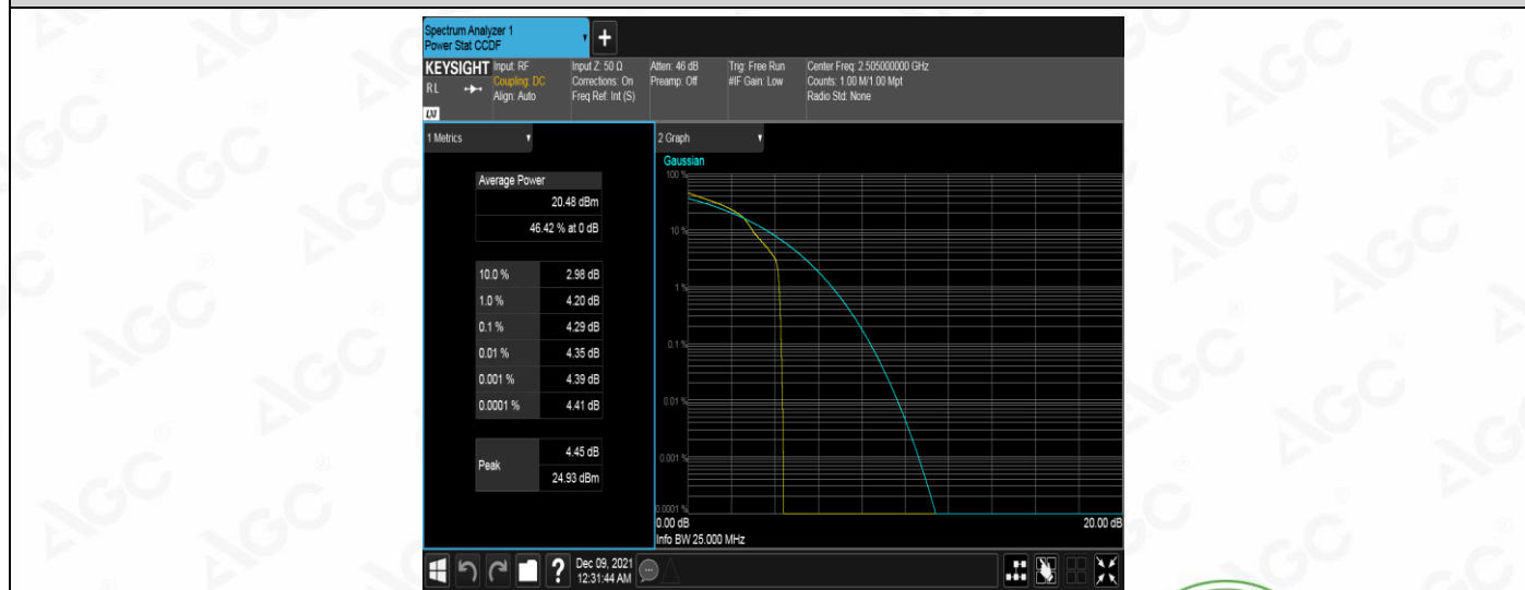
Band7-10MHz-16QAM-20800-1RB#0
