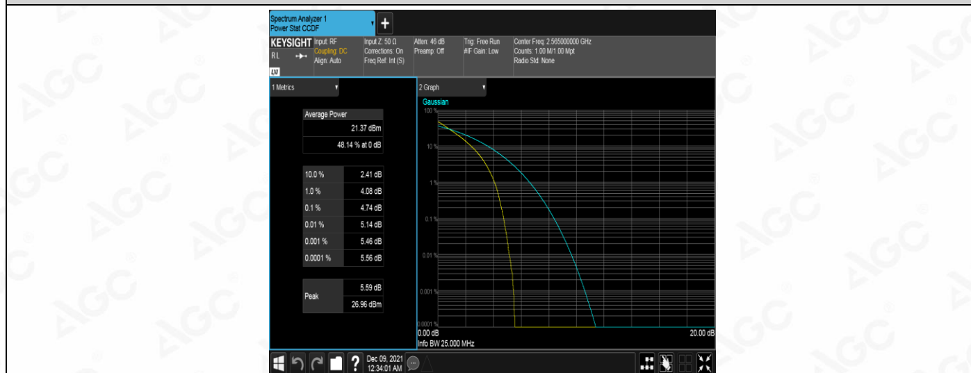
Band7-10MHz-16QAM-20800-1RB#0
