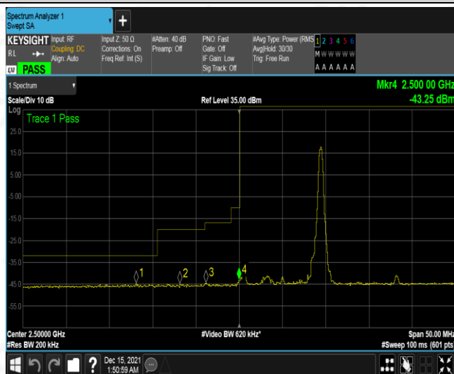
Band7-10MHz-16QAM-20800-1RB#49
