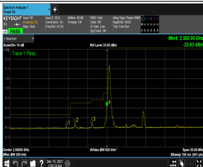
Band7-10MHz-16QAM-20800-1RB#49
