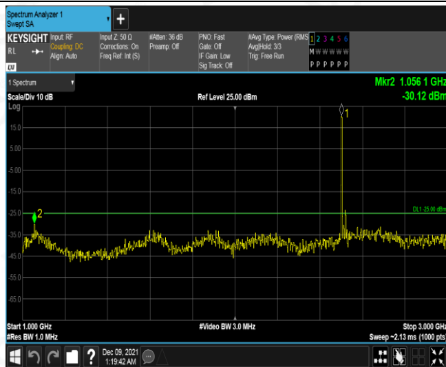
Band7-20MHz-16QAM-20850-1RB#0-Range2:1000~3000MHz
