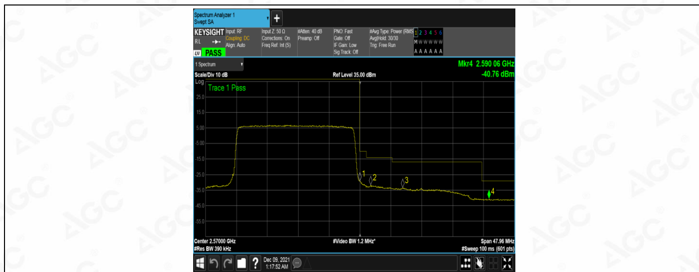
Band7-20MHz-16QAM-20850-1RB#0
