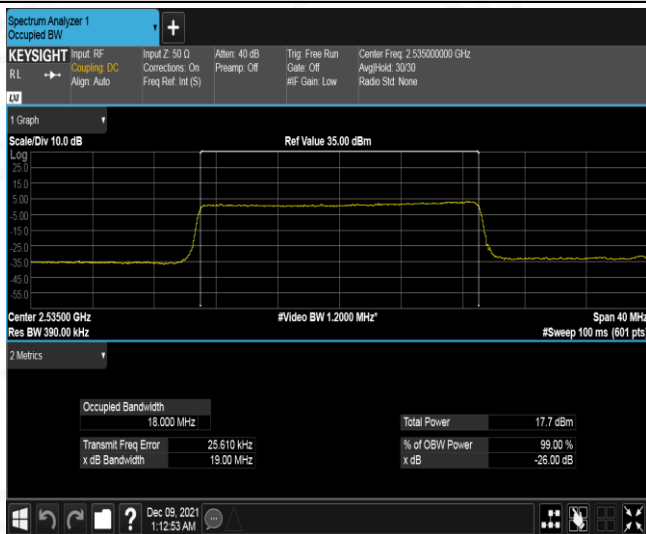
Band7-20MHz-QPSK-21100-100RB#0
