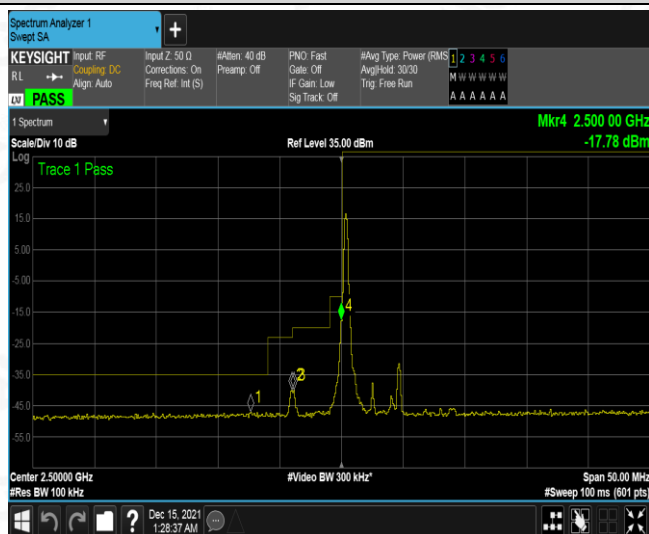
Band7-5MHz-QPSK-20775-1RB#24
