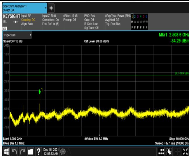
Band5-1.4MHz-16QAM-20525-1RB#0-Range2:1000~10000MHz
