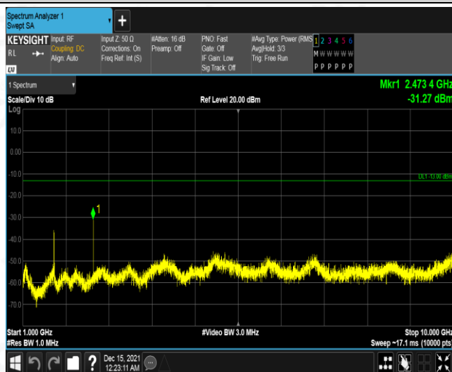
Band5-3MHz-16QAM-20415-1RB#0-Range2:1000~10000MHz
