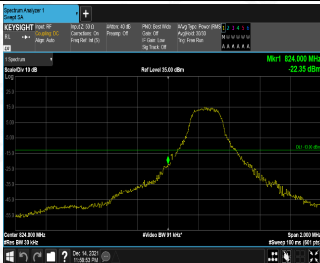
Band5-1.4MHz-QPSK-20407-1RB#5
