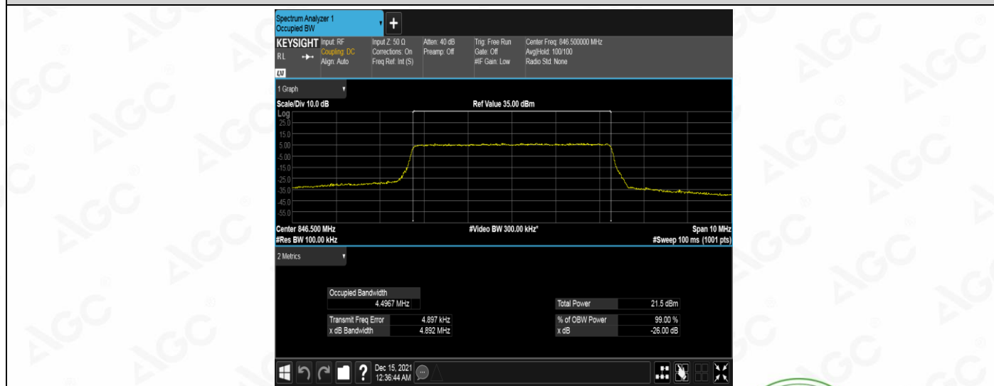
Band5-5MHz-QPSK-20625-25RB#0
