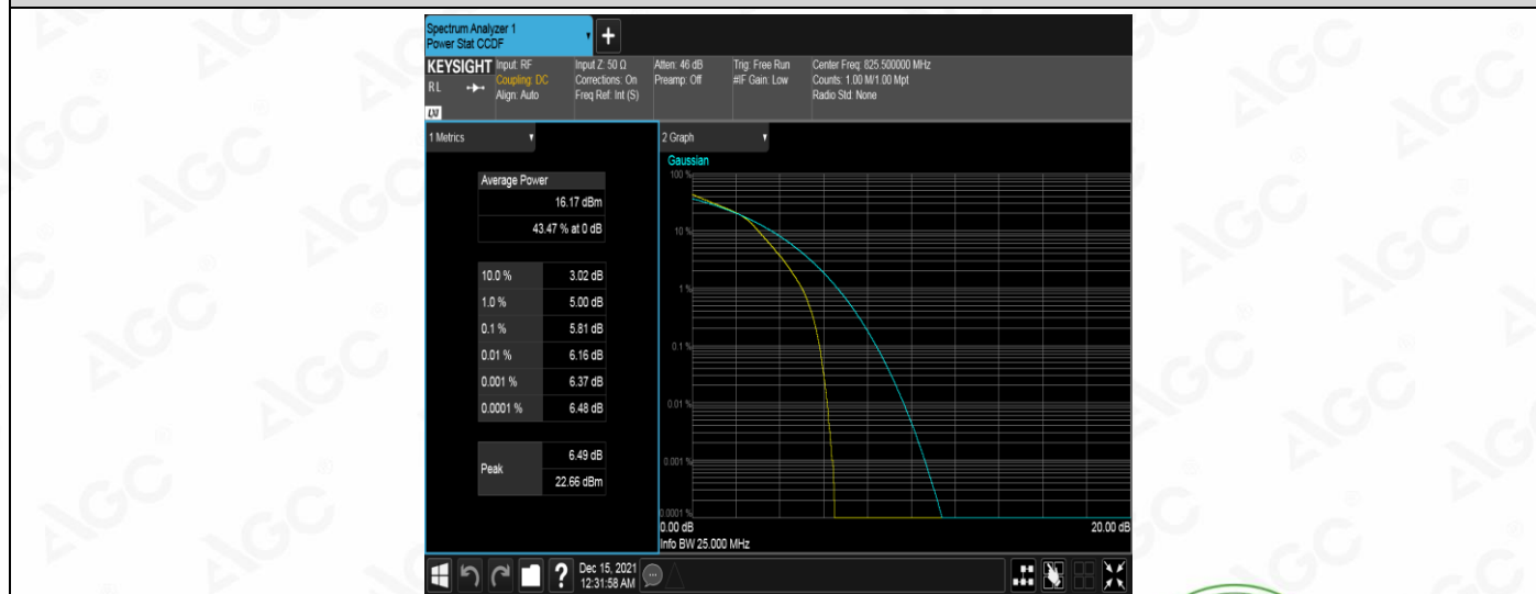
Band5-3MHz-16QAM-20415-15RB#0
