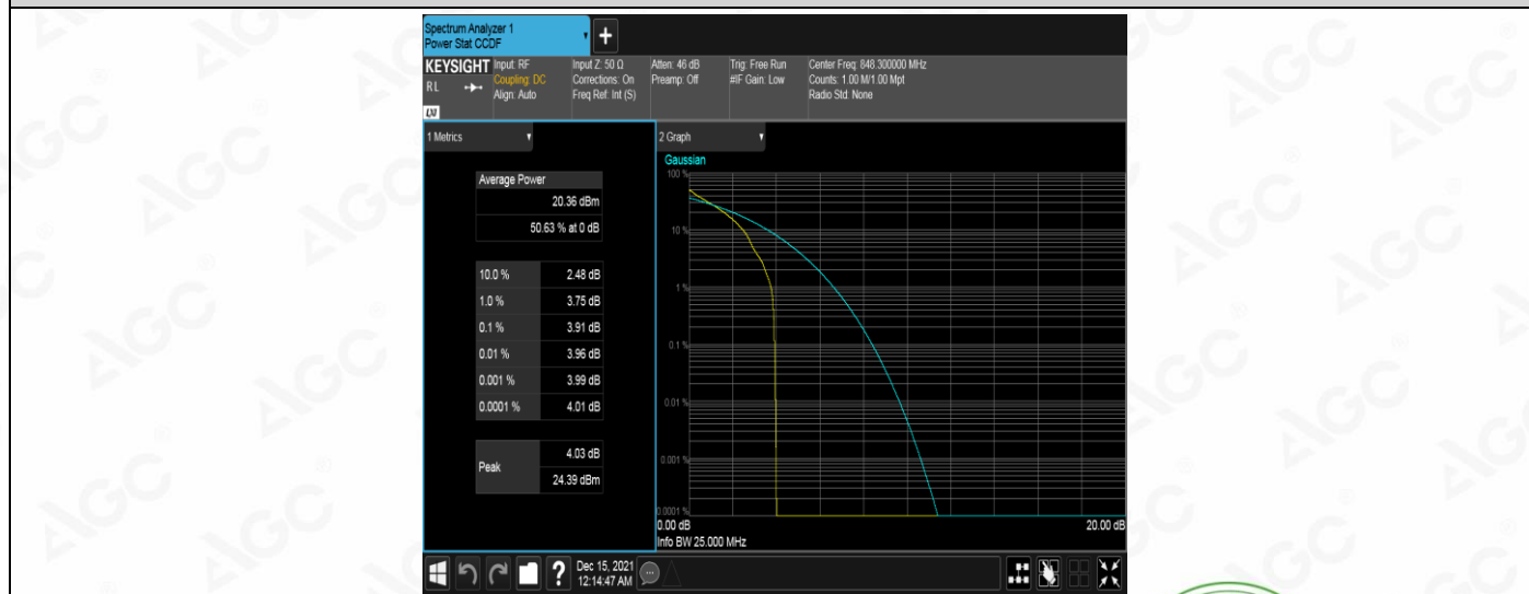
Band5-1.4MHz-QPSK-20643-1RB#0
