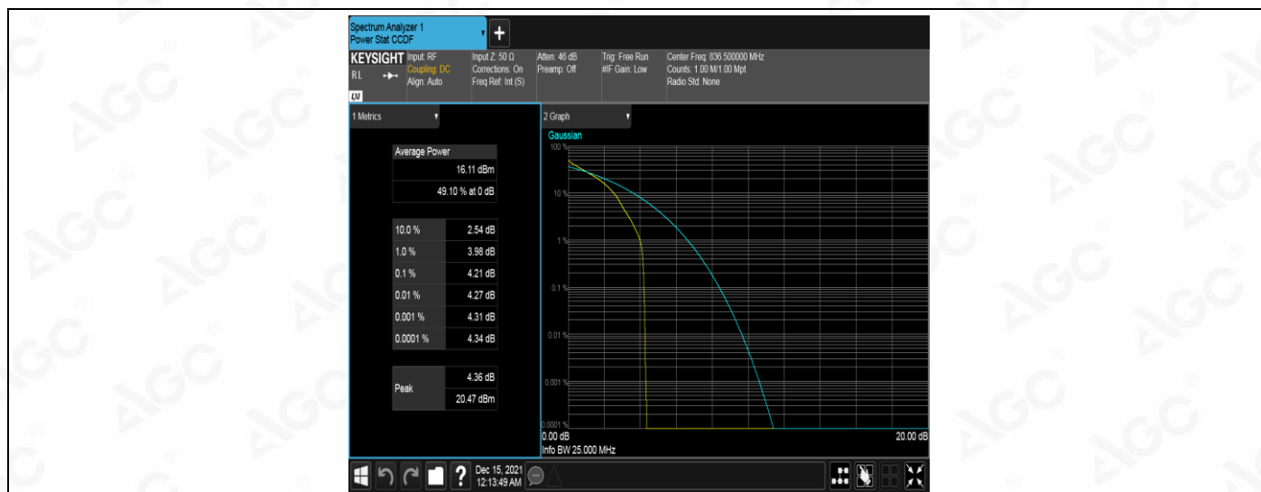
Band5-1.4MHz-QPSK-20525-6RB#0
