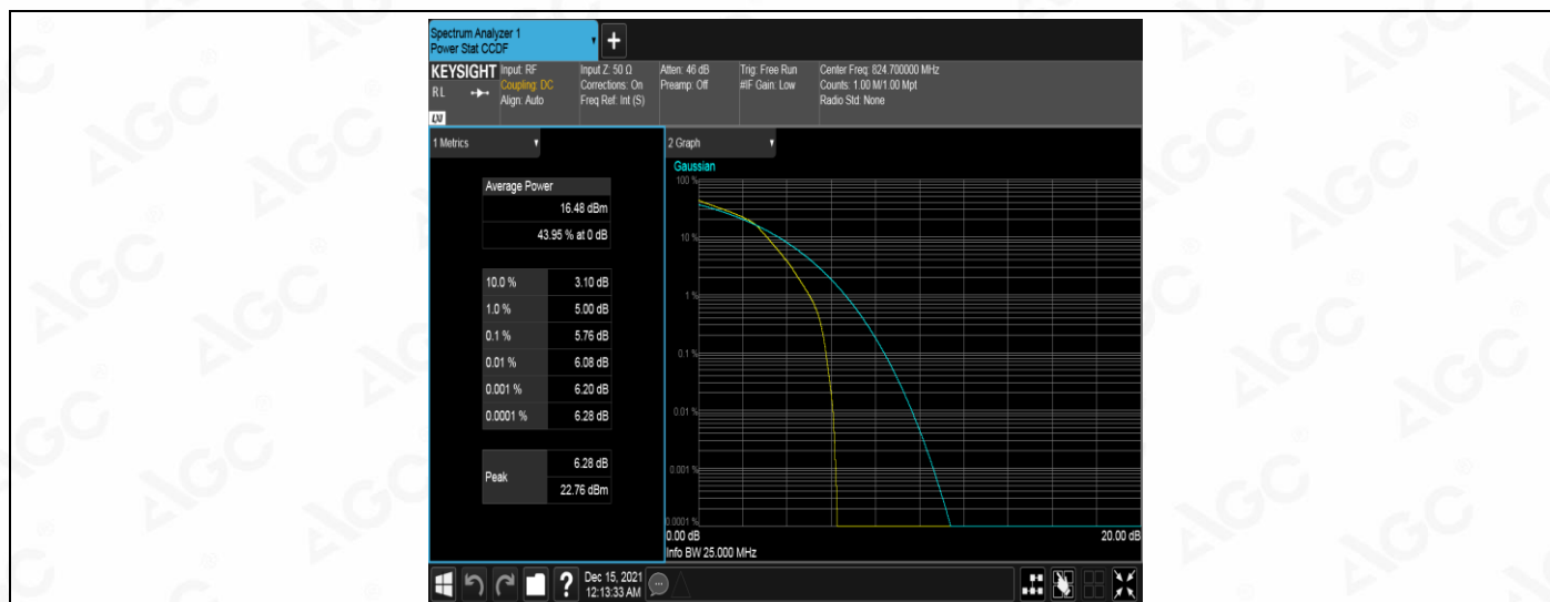
Band5-1.4MHz-16QAM-20525-1RB#0
