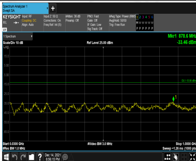
Band2-10MHz-QPSK-18650-1RB#0-Range1:30~1000MHz
