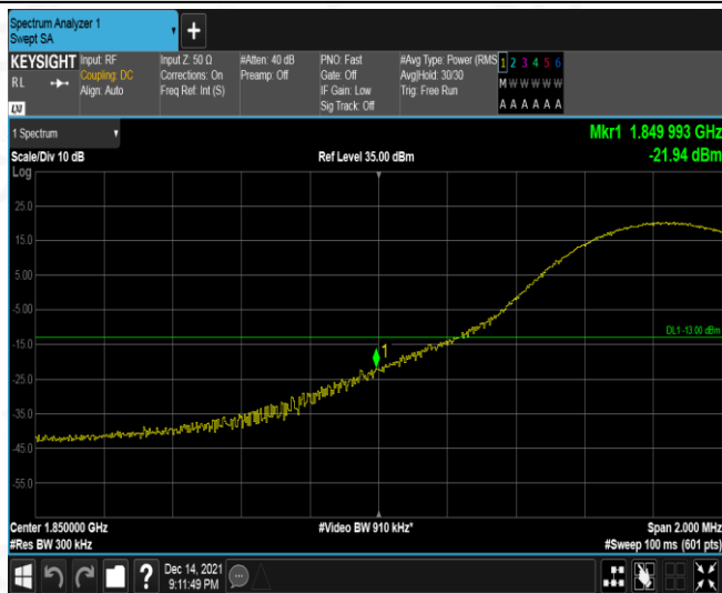
Band2-15MHz-16QAM-18675-1RB#0
