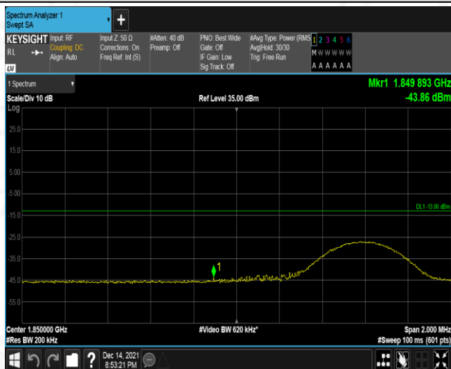
Band2-10MHz-16QAM-18650-50RB#0
