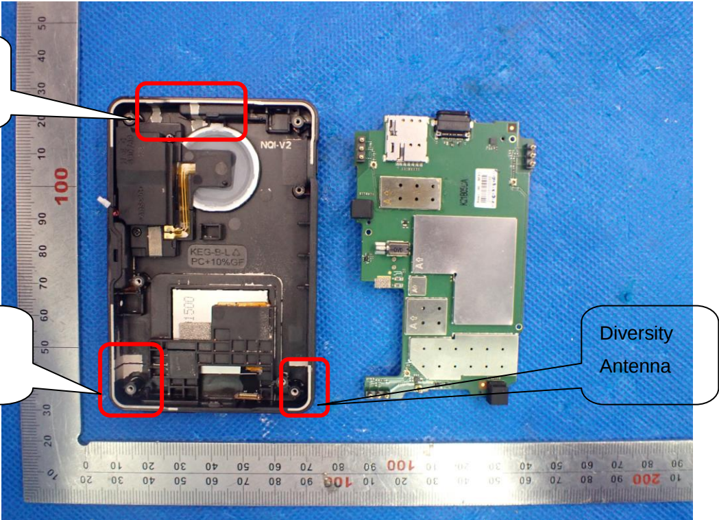
OPEN VIEW OF EUT(FIGURE 3)
