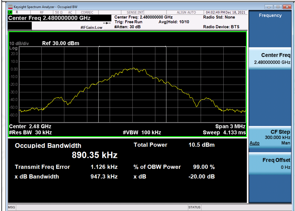
Test_Graph_BR_ANT1_2480_1Mbps_OBW
