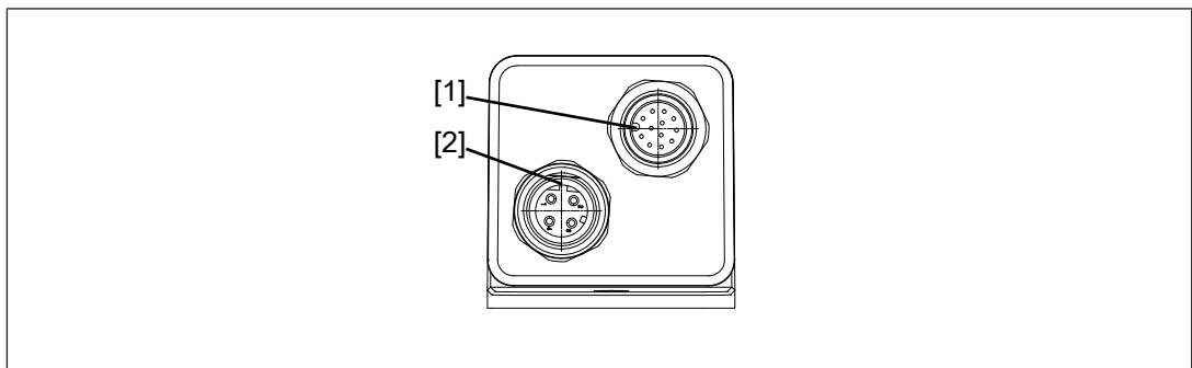
Fig.: View of the PIT gb with PITreader from the connector end: Position of the coding elements on the connectors to protect the cables from twisting.
