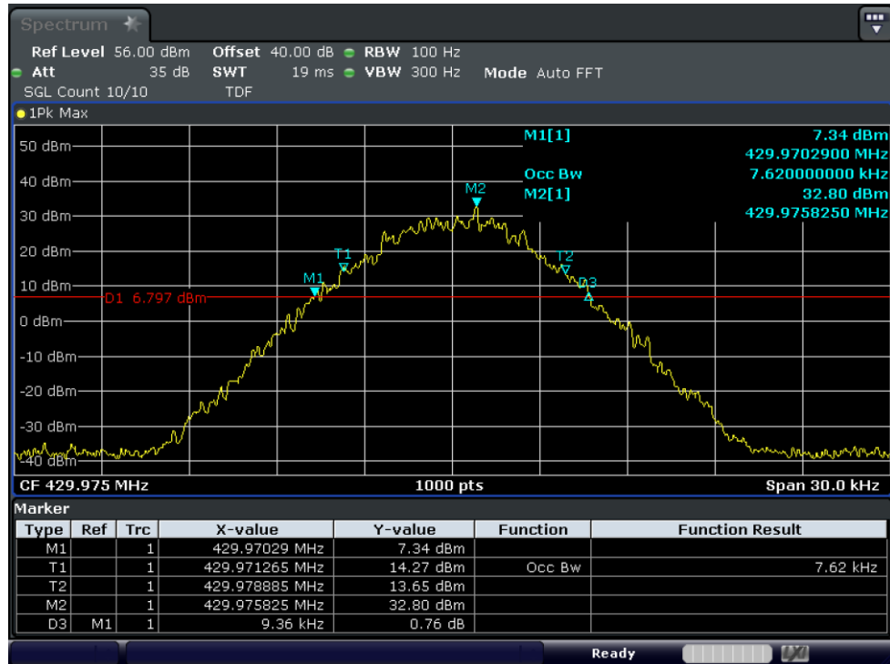
Test Graph 4FSK Data 5W 429.975 12.5k OBW
