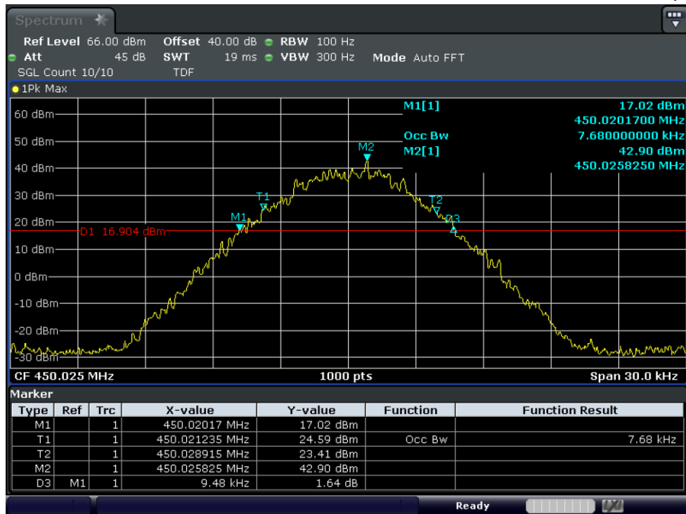
Test Graph 4FSK Data+Voice 50W 450.025 12.5k OBW
