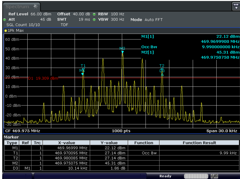
Test Graph FM 50W 469.975 12.5k OBW
