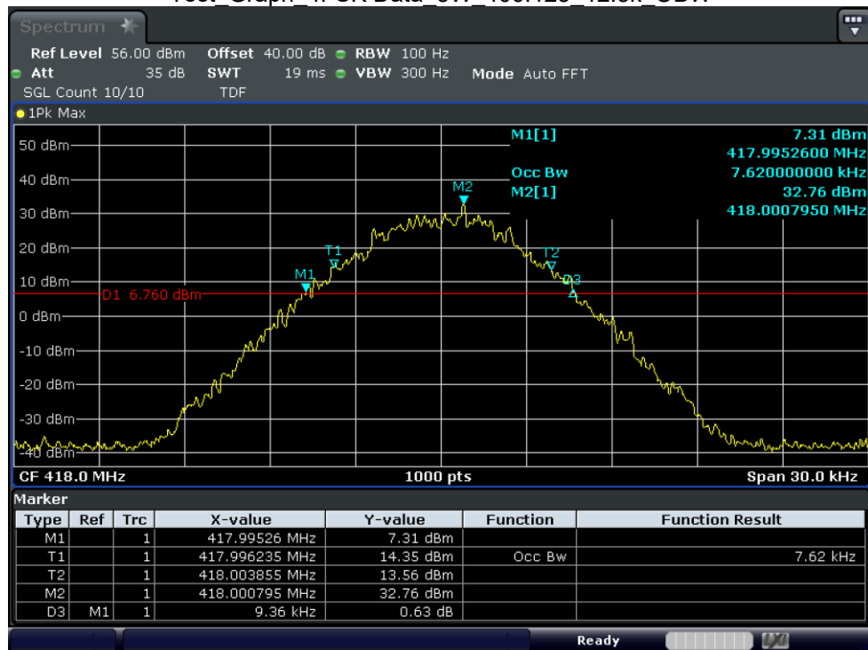
Test_Graph_4FSK Data_5W_418_12.5k_OBW
