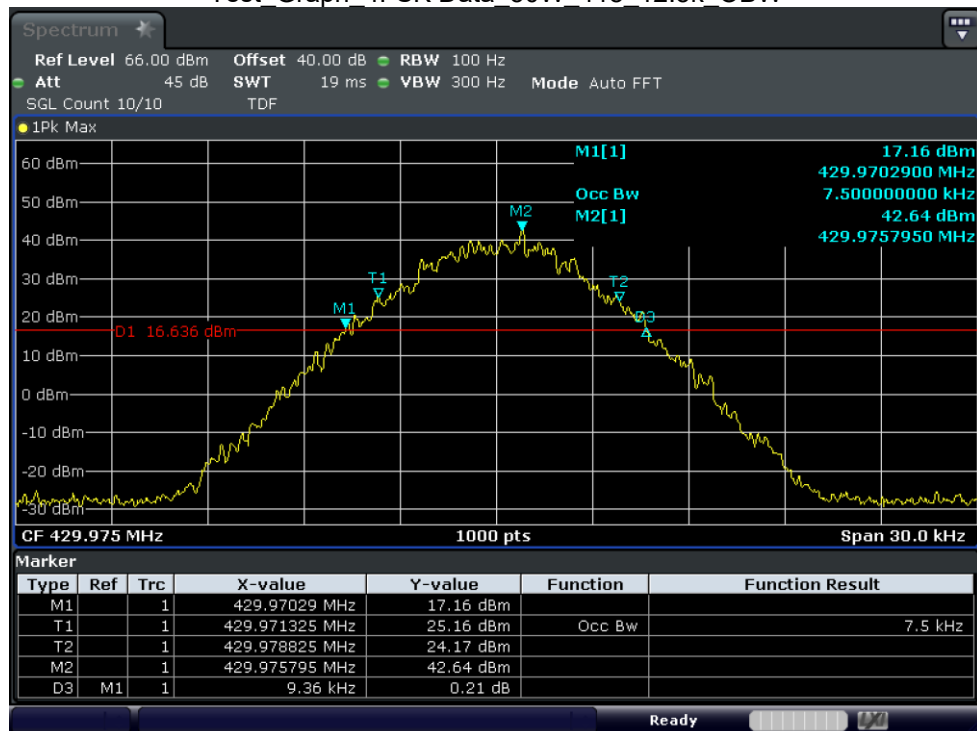
Test_Graph_4FSK Data_50W_429.975_12.5k_OBW
