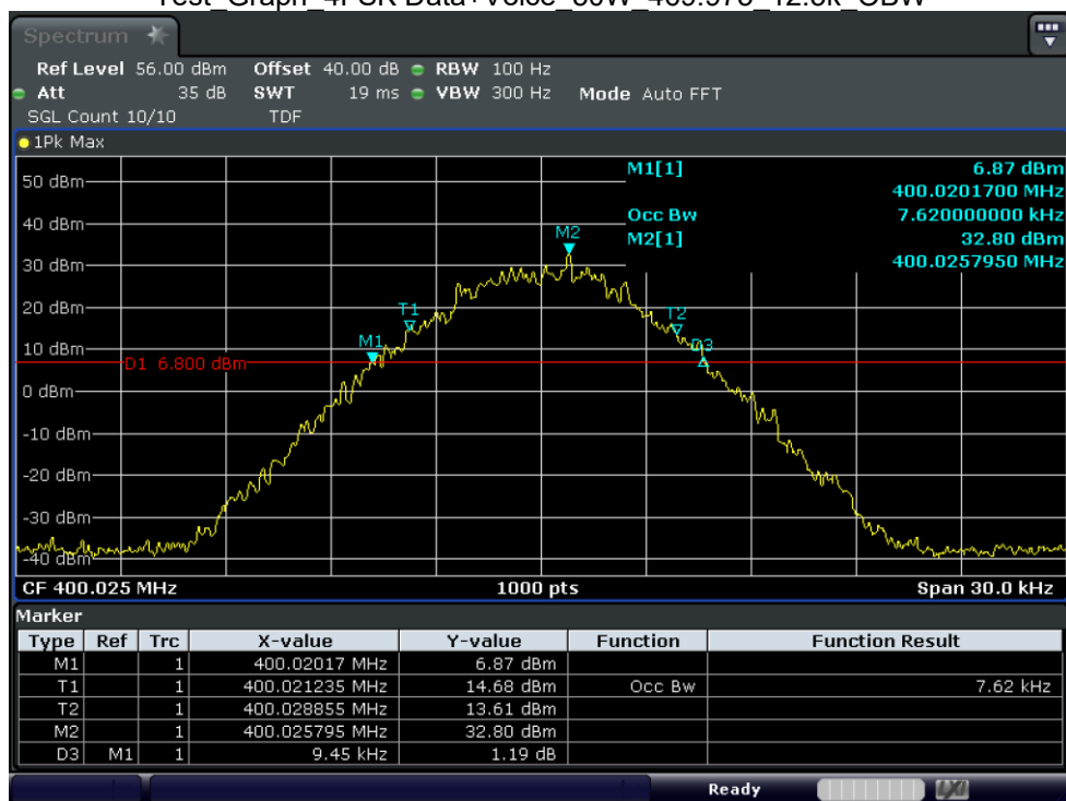
Test_Graph_4FSK Data+Voice_5W_400.025_12.5k_OBW
