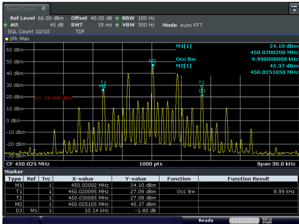
Test Graph FM 50W 450.025 12.5k OBW
