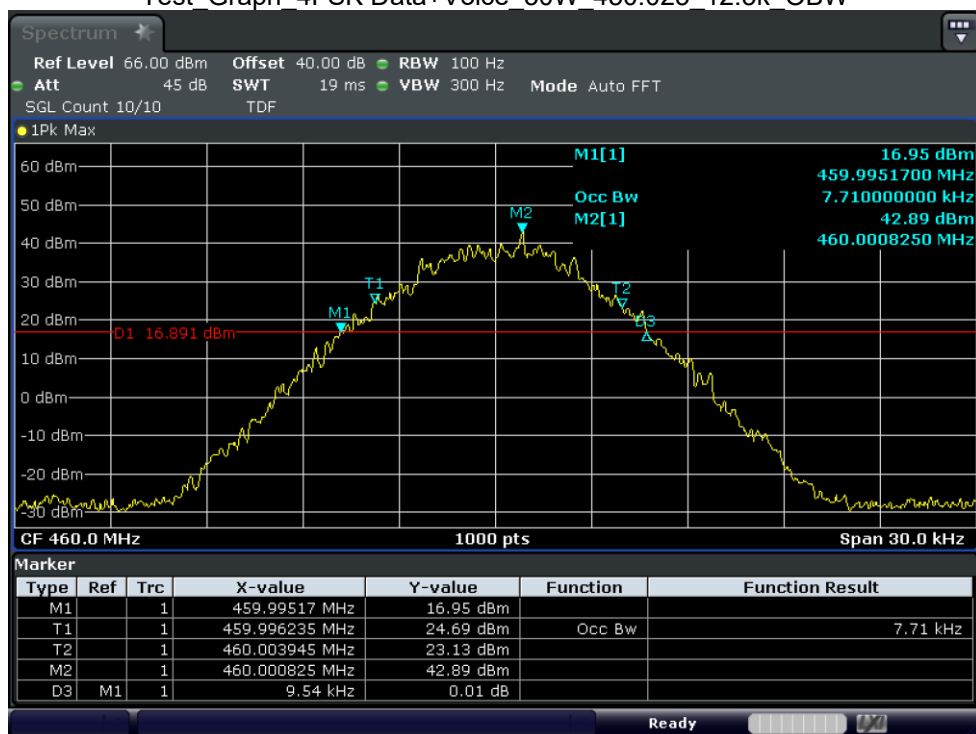
Test_Graph_4FSK Data+Voice_50W_460_12.5k_OBW
