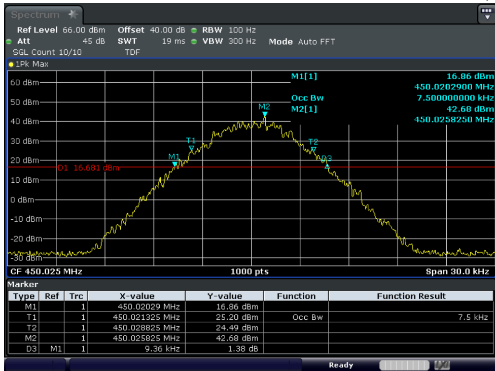
Test Graph 4FSK Data 50W 450.025 12.5k OBW
