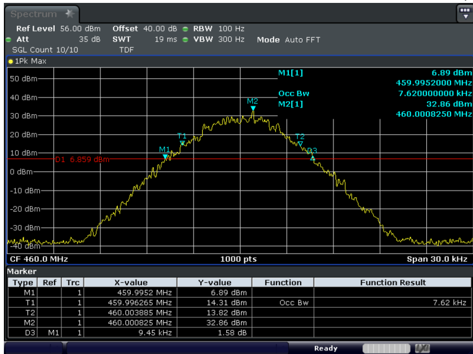
Test Graph 4FSK Data 5W 460 12.5k OBW
