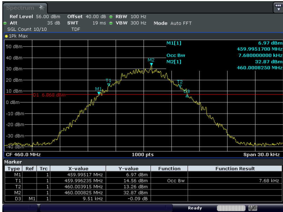
Test Graph 4FSK Data+Voice 5W 460 12.5k OBW
