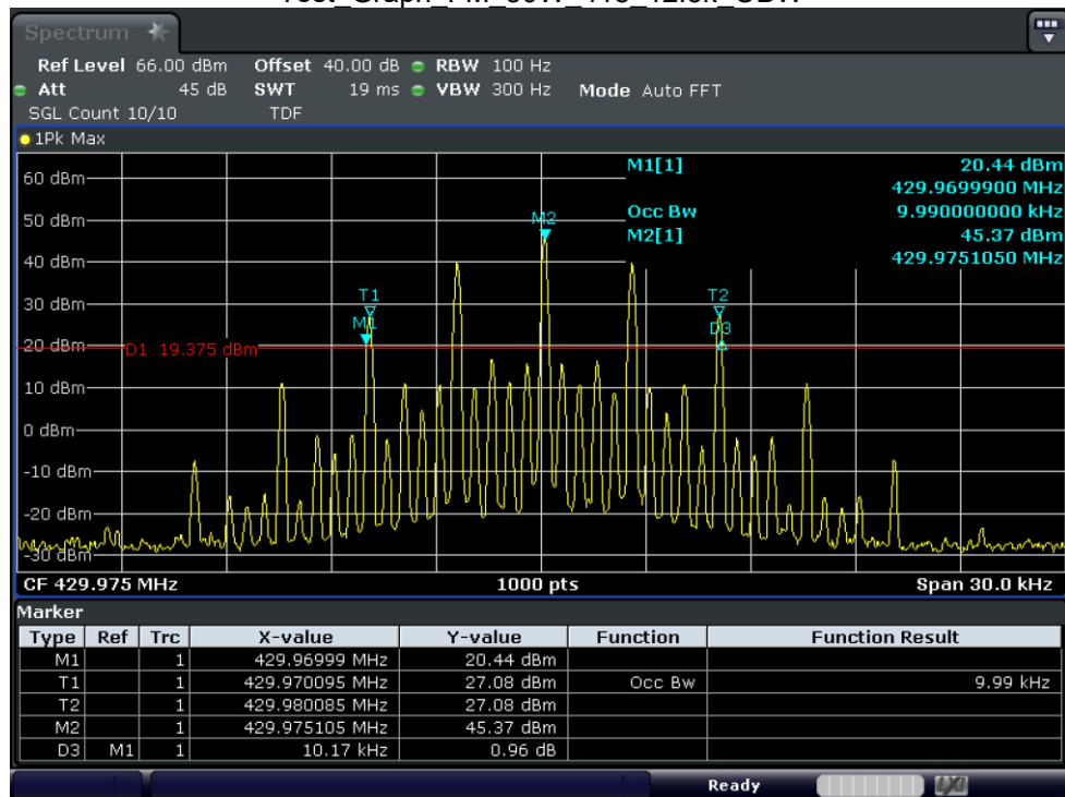
Test_Graph_FM_50W_429.975_12.5k_OBW
