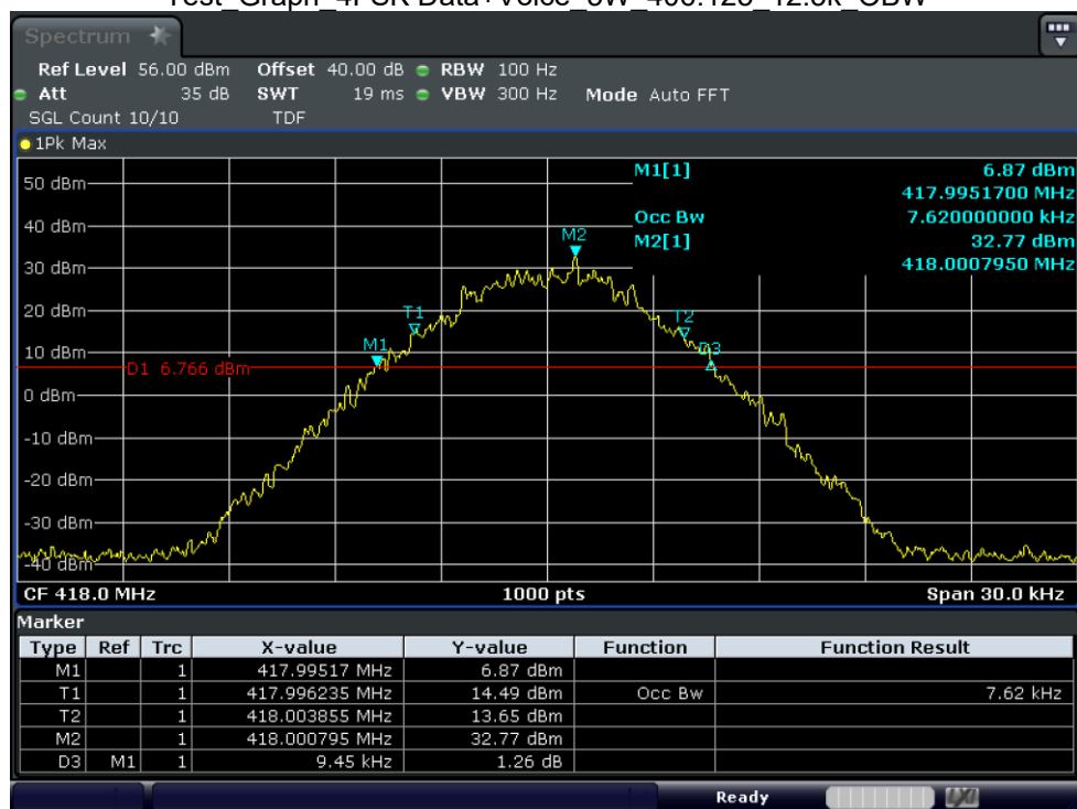
Test_Graph_4FSK Data+Voice_5W_418_12.5k_OBW
