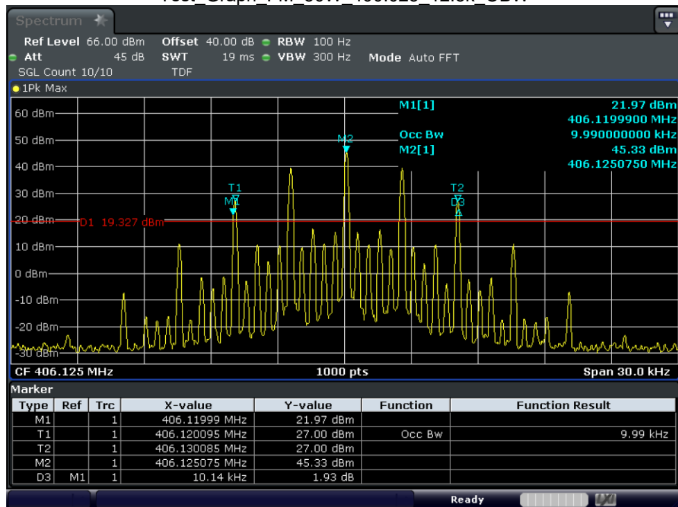
Test_Graph_FM_50W_406.125_12.5k_OBW
