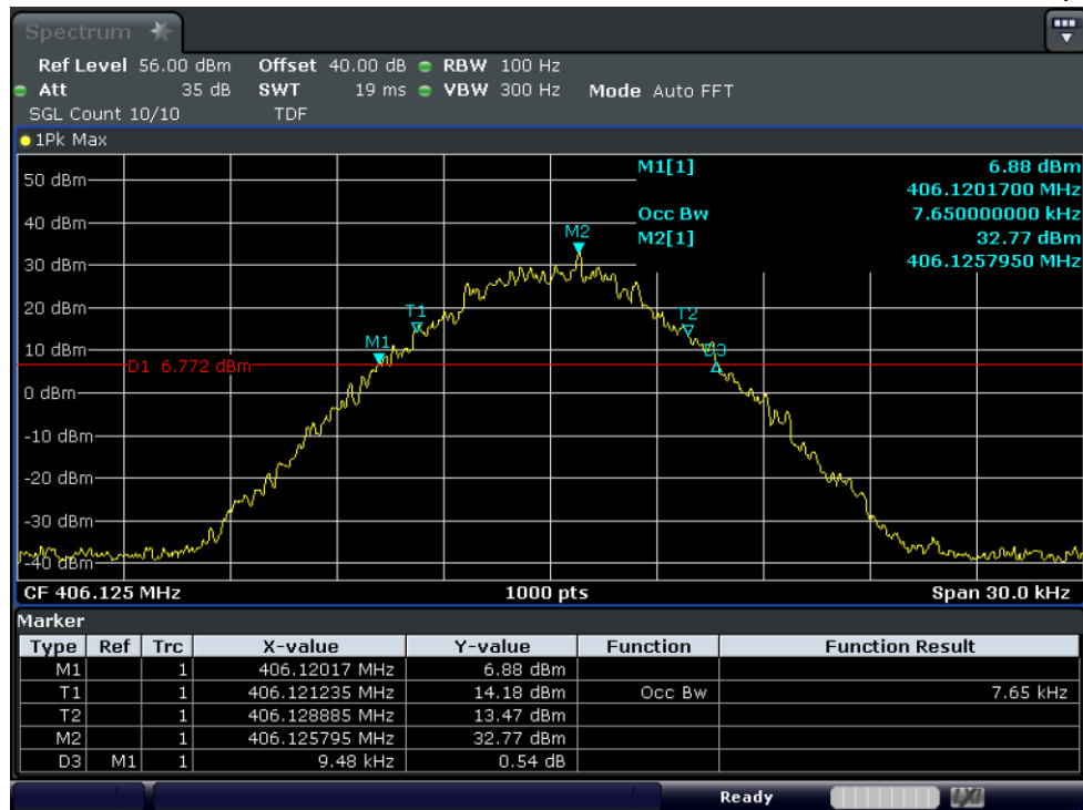
Test Graph 4FSK Data+Voice 5W 406.125 12.5k OBW
