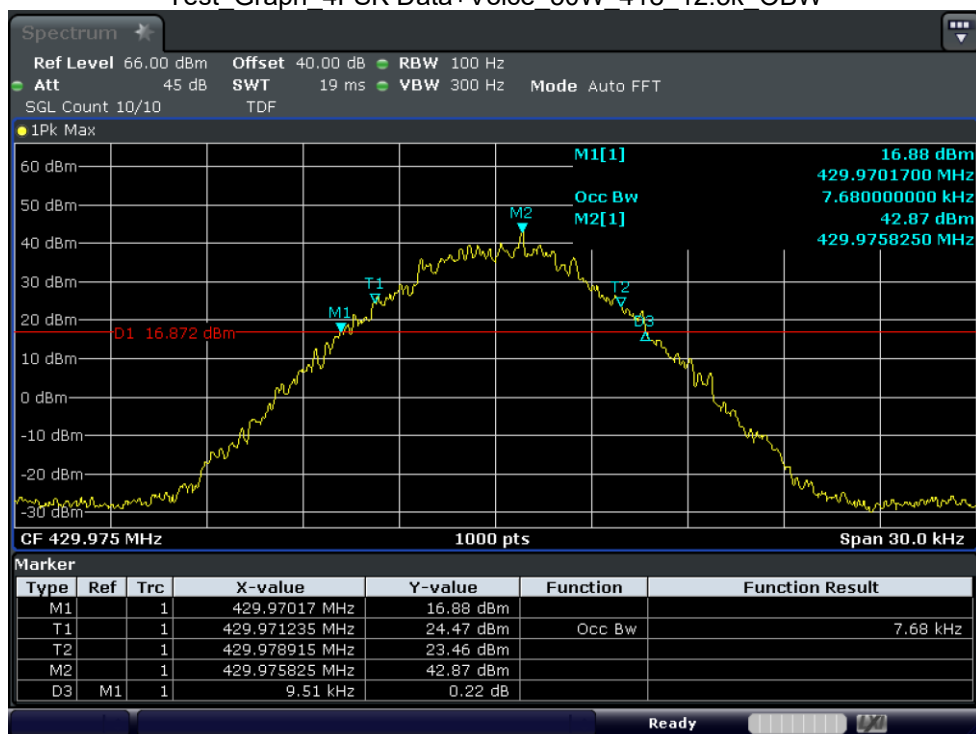
Test_Graph_4FSK Data+Voice_50W_429.975_12.5k_OBW
