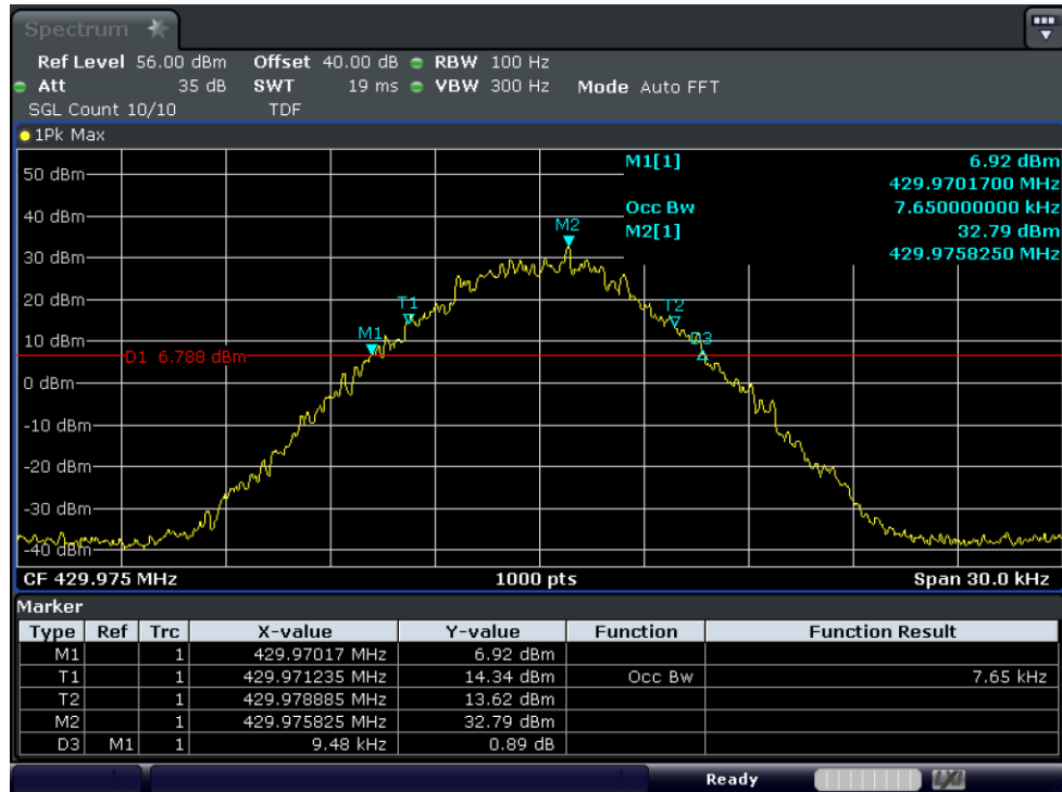
Test Graph 4FSK Data+Voice 5W 429.975 12.5k OBW
