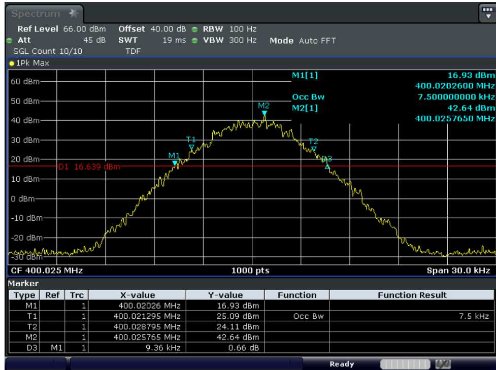
Test Graph 4FSK Data 50W 400.025 12.5k OBW
