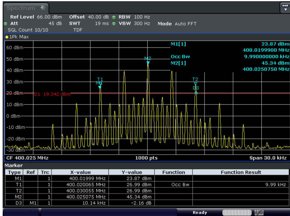
Test Graph FM 50W 400.025 12.5k OBW
