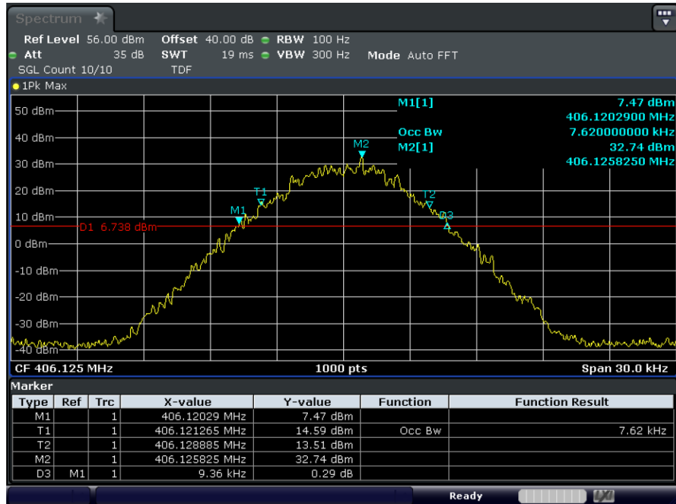
Test Graph 4FSK Data 5W 406.125 12.5k OBW
