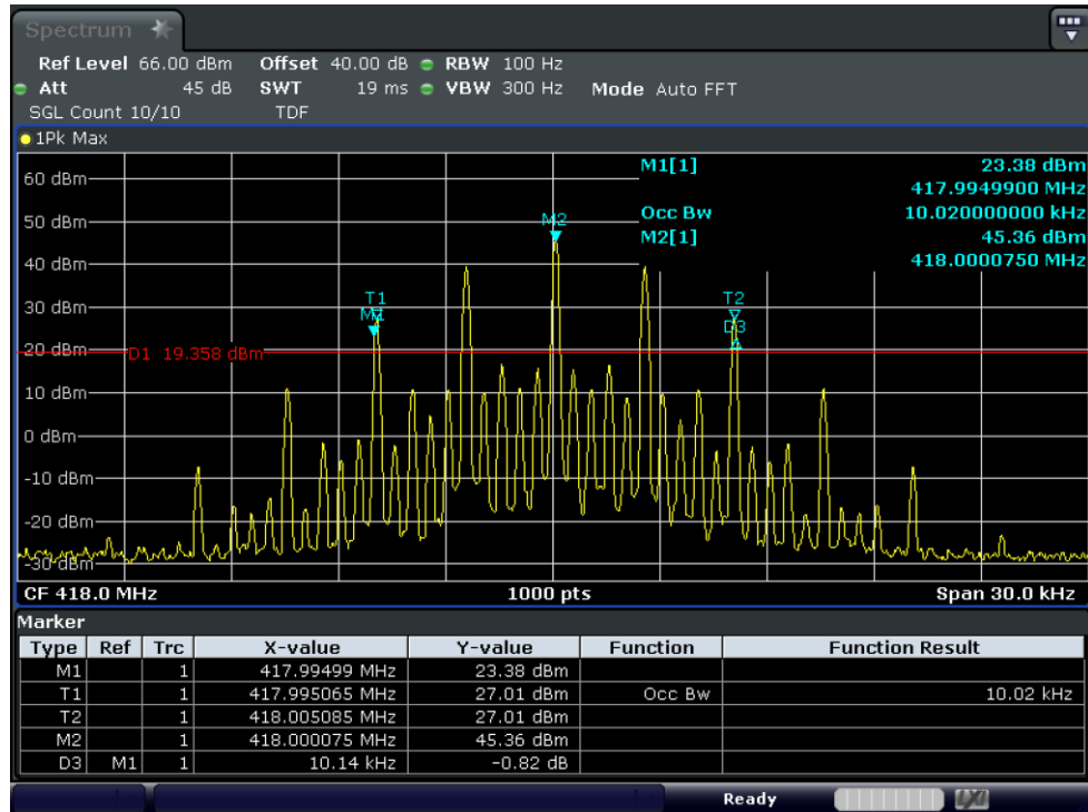
Test Graph FM 50W 418 12.5k OBW
