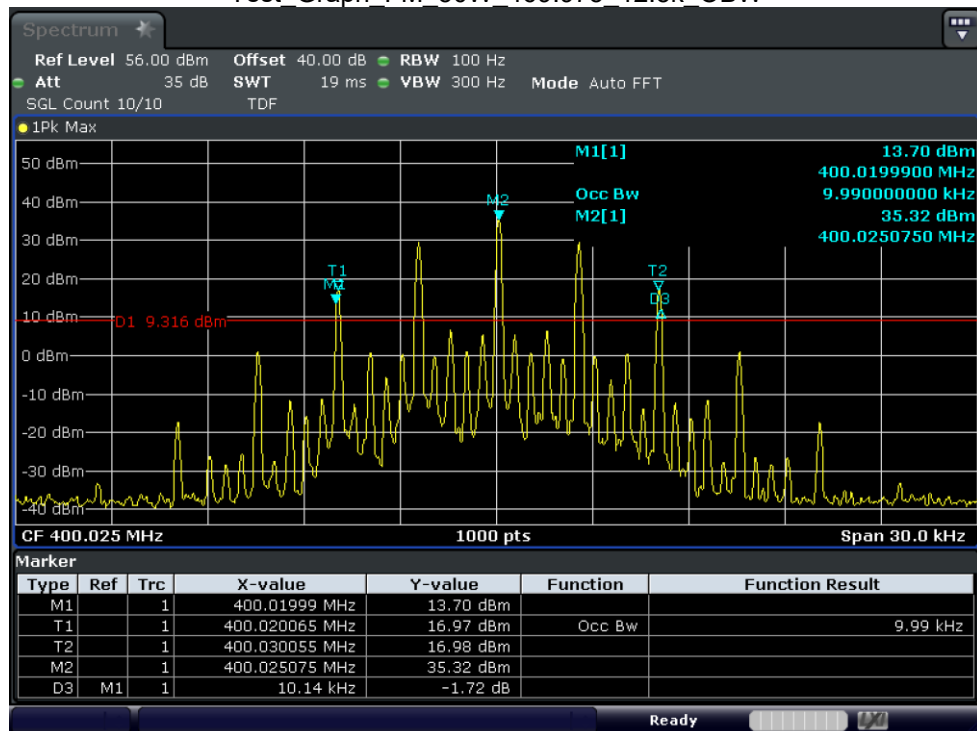
Test_Graph_FM_5W_400.025_12.5k_OBW
