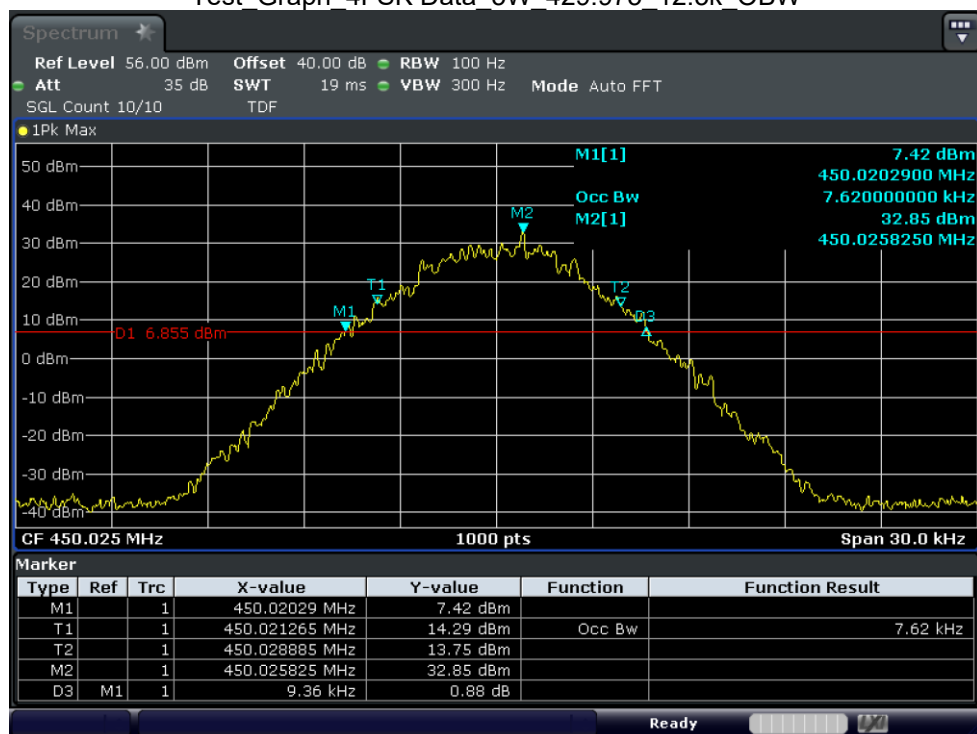
Test_Graph_4FSK Data_5W_450.025_12.5k_OBW
