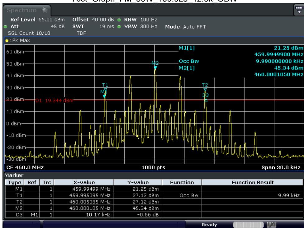
Test_Graph_FM_50W_460_12.5k_OBW
