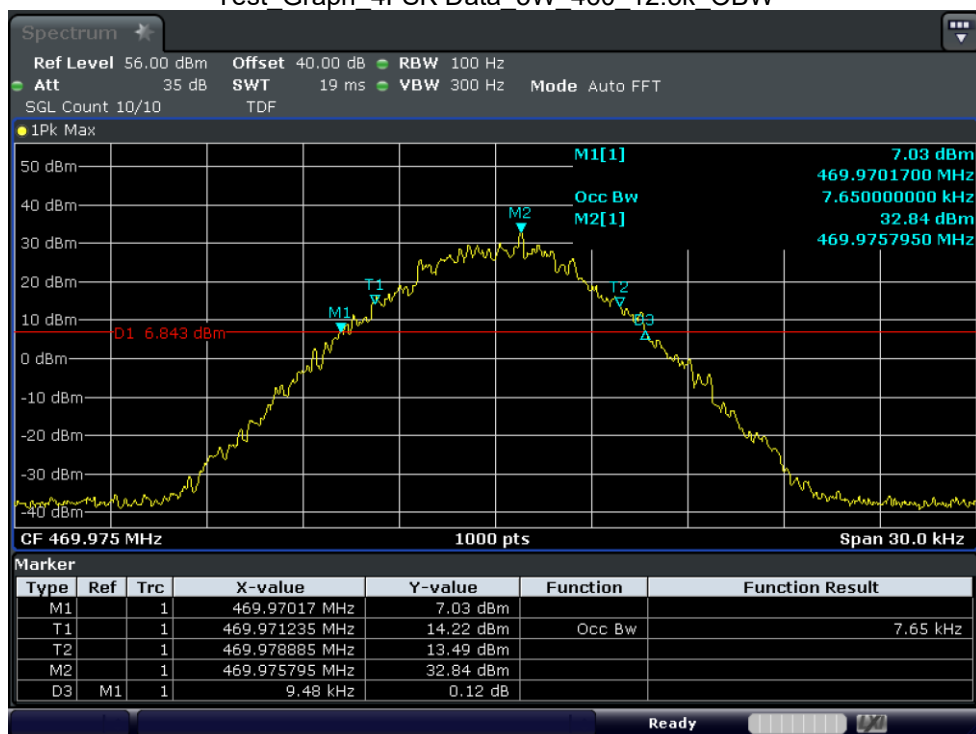
Test_Graph_4FSK Data_5W_469.975_12.5k_OBW
