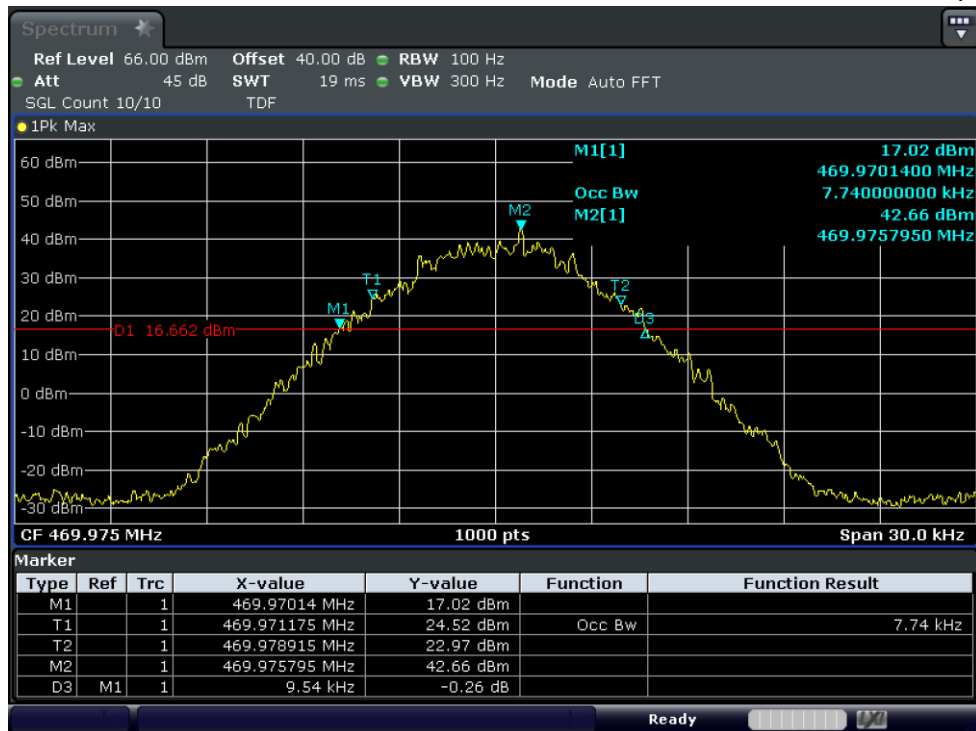
Test Graph 4FSK Data+Voice 50W 469.975 12.5k OBW
