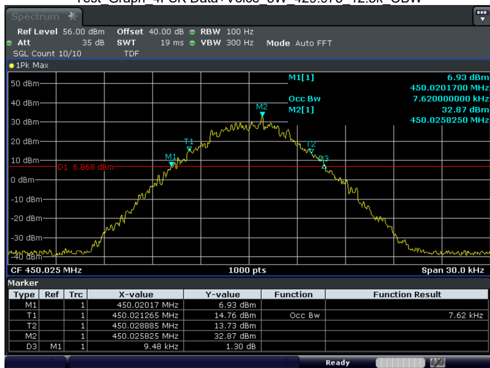
Test_Graph_4FSK Data+Voice_5W_450.025_12.5k_OBW
