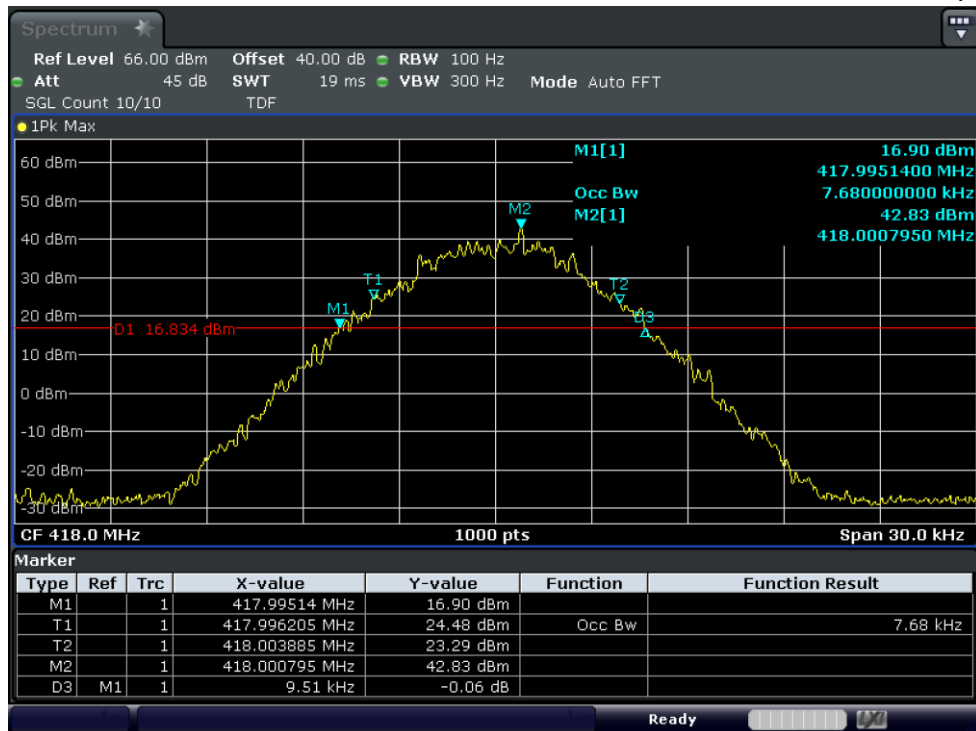
Test Graph 4FSK Data+Voice 50W 418 12.5k OBW
