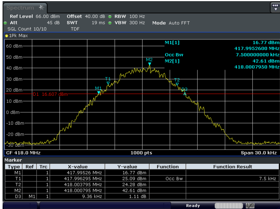
Test Graph 4FSK Data 50W 418 12.5k OBW
