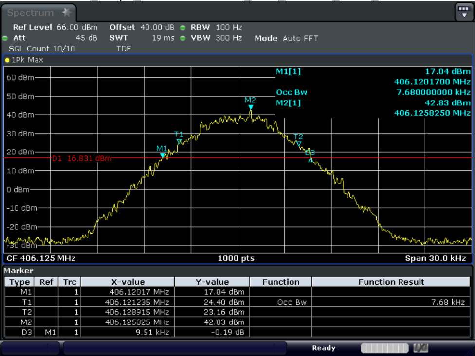
Test_Graph_4FSK Data+Voice_50W_406.125_12.5k_OBW
