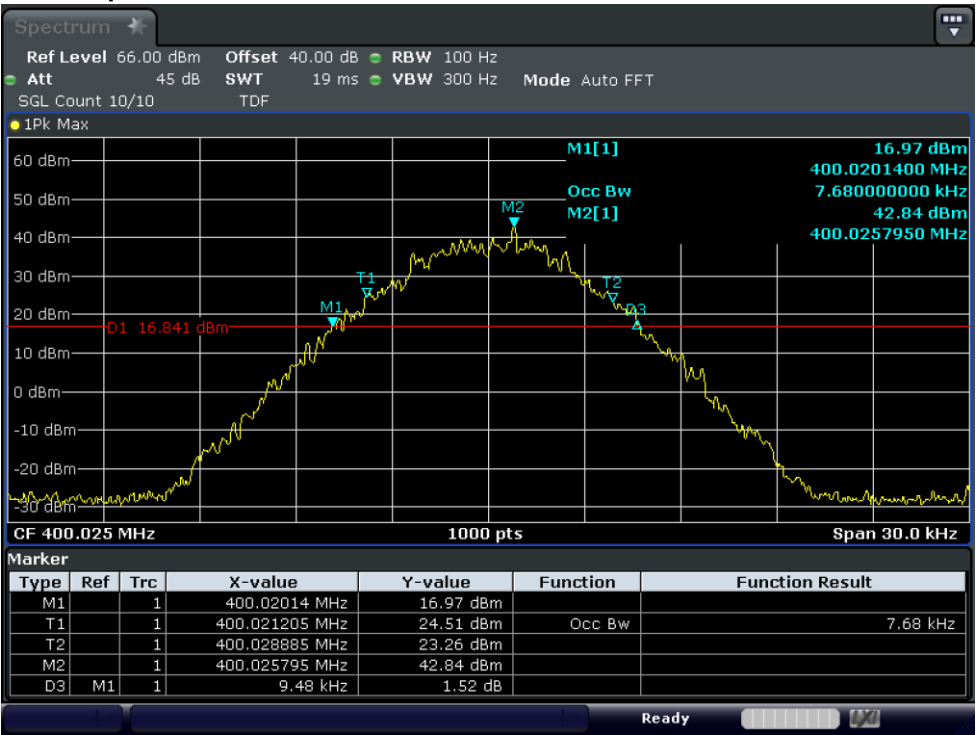
Test Graph 4FSK Data+Voice 50W 400.025 12.5k OBW
