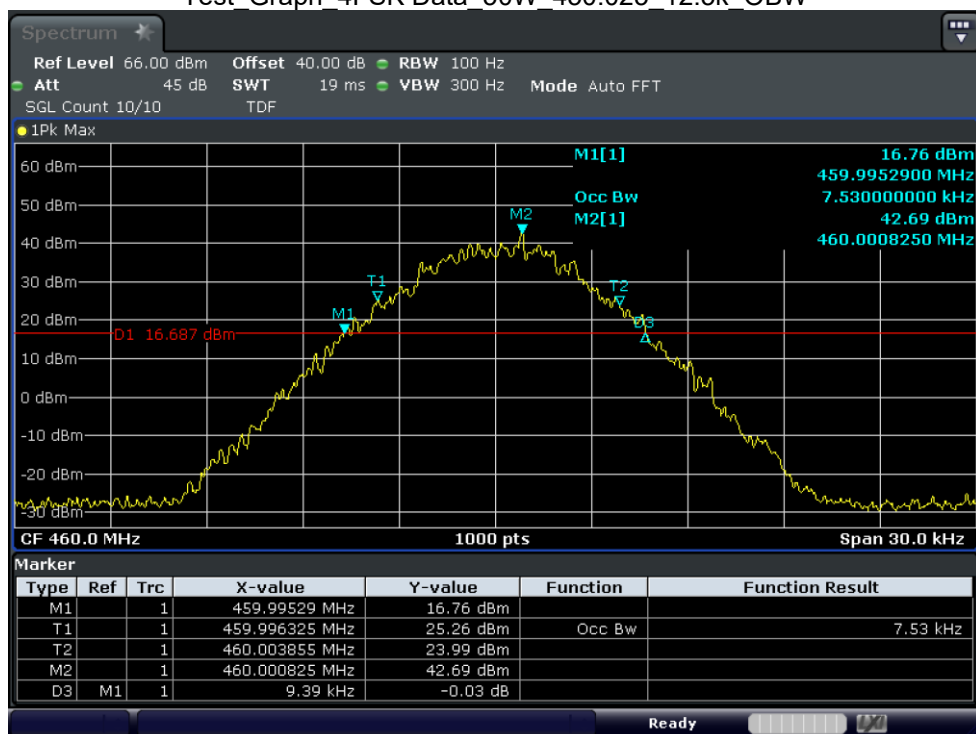
Test_Graph_4FSK Data_50W_460_12.5k_OBW
