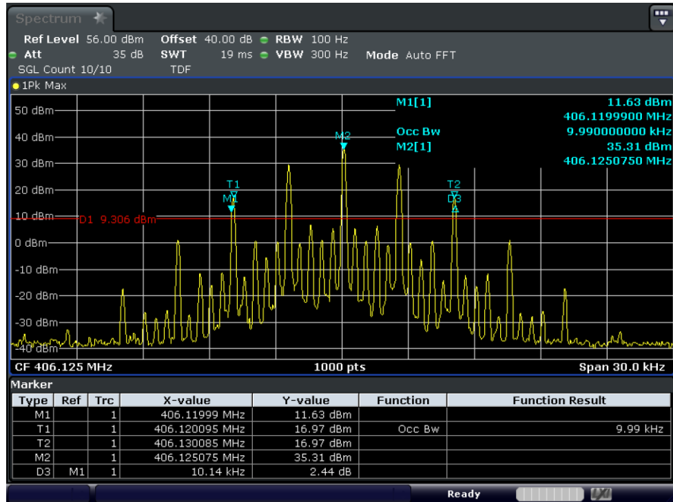
Test Graph FM 5W 406.125 12.5k OBW
