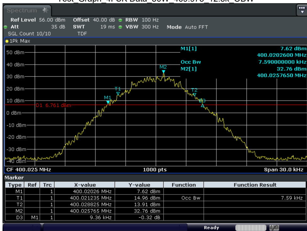
Test_Graph_4FSK Data_5W_400.025_12.5k_OBW
