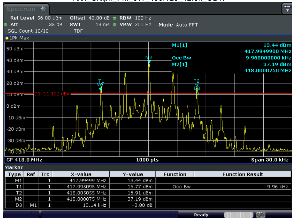
Test_Graph_FM_5W_418_12.5k_OBW
