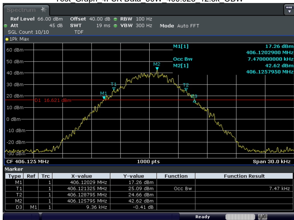
Test_Graph_4FSK Data_50W_406.125_12.5k_OBW
