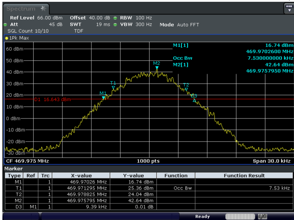
Test Graph 4FSK Data 50W 469.975 12.5k OBW
