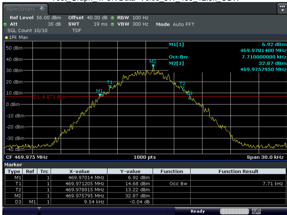
Test_Graph_4FSK Data+Voice_5W_469.975_12.5k_OBW
