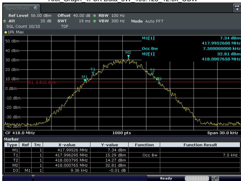
Test_Graph_4FSK Data_5W_418_12.5k_OBW
