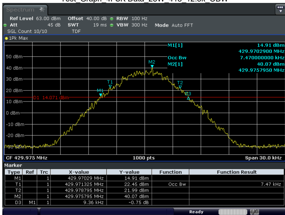
Test_Graph_4FSK Data_25W_429.975_12.5k_OBW
