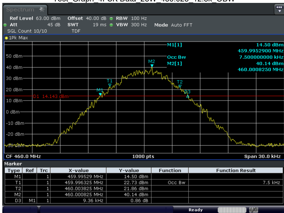
Test_Graph_4FSK Data_25W_460_12.5k_OBW
