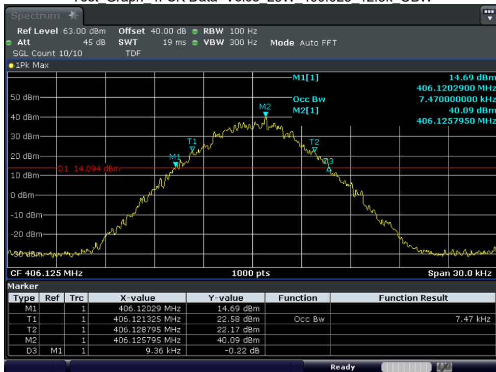
Test_Graph_4FSK Data+Voice_25W_406.125_12.5k_OBW
