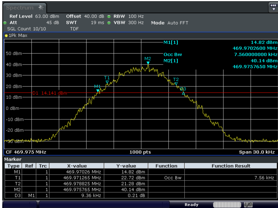
Test Graph 4FSK Data+Voice 25W 469.975 12.5k OBW
