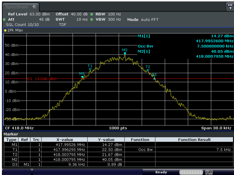
Test Graph 4FSK Data 25W 418 12.5k OBW
