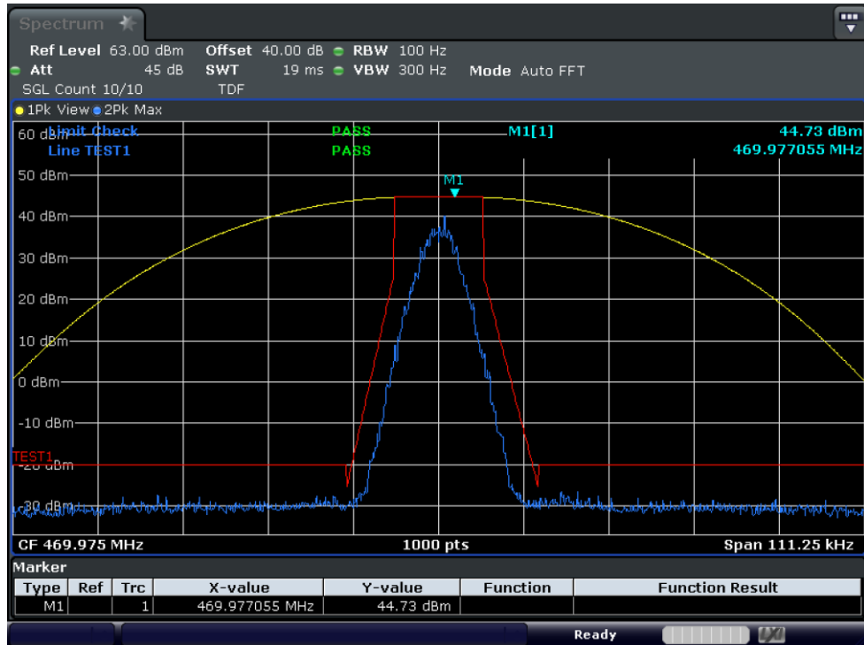
Test Graph 4FSK Data+Voice 25W 469.975 12.5k Mask D
