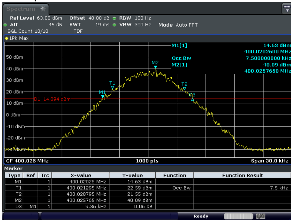
Test Graph 4FSK Data+Voice 25W 400.025 12.5k OBW
