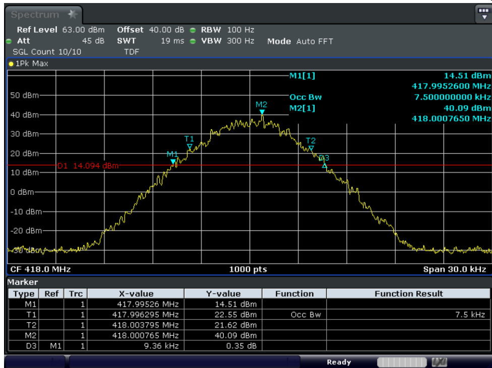
Test Graph 4FSK Data+Voice 25W 418 12.5k OBW
