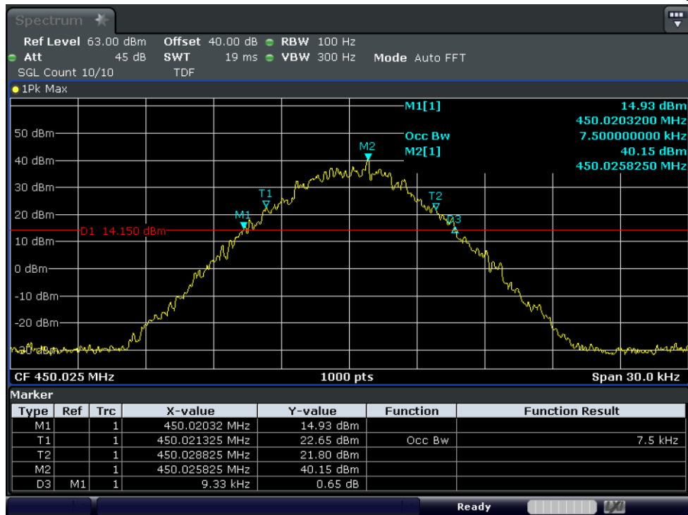
Test Graph 4FSK Data 25W 450.025 12.5k OBW
