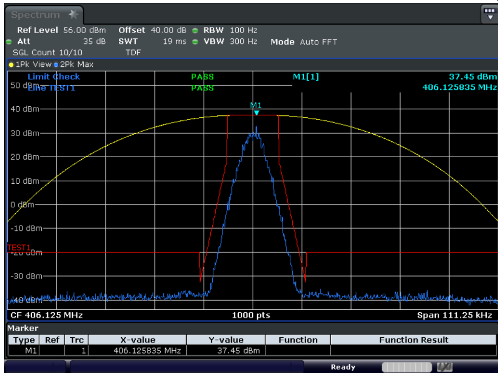
Test Graph 4FSK Data+Voice 5W 406.125 12.5k Mask D
