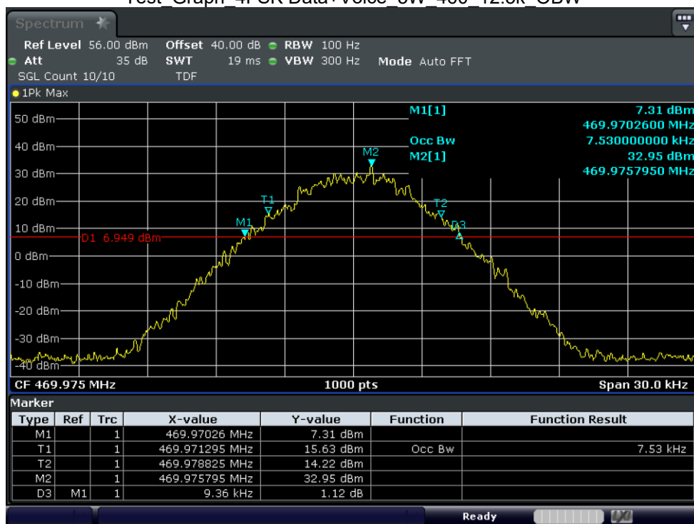
Test_Graph_4FSK Data+Voice_5W_469.975_12.5k_OBW
