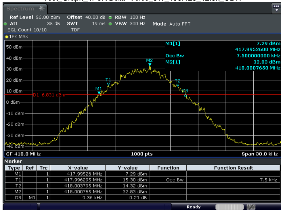
Test_Graph_4FSK Data+Voice_5W_418_12.5k_OBW
