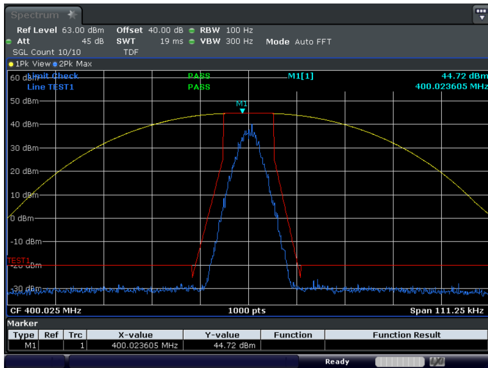
Test Graph 4FSK Data+Voice 25W 400.025 12.5k Mask D
