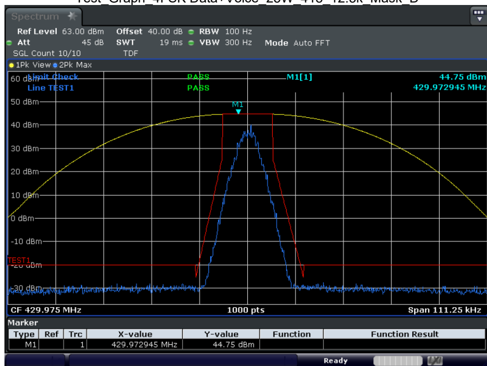
Test_Graph_4FSK Data+Voice_25W_429.975_12.5k_Mask_D
