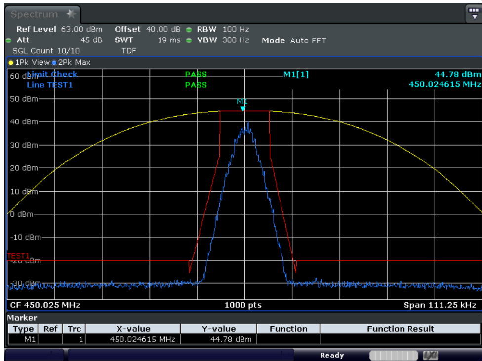
Test Graph_4FSK Data+Voice_25W_450.025_12.5k_Mask_D
