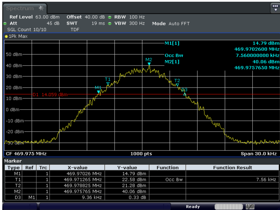
Test Graph 4FSK Data 25W 469.975 12.5k OBW
