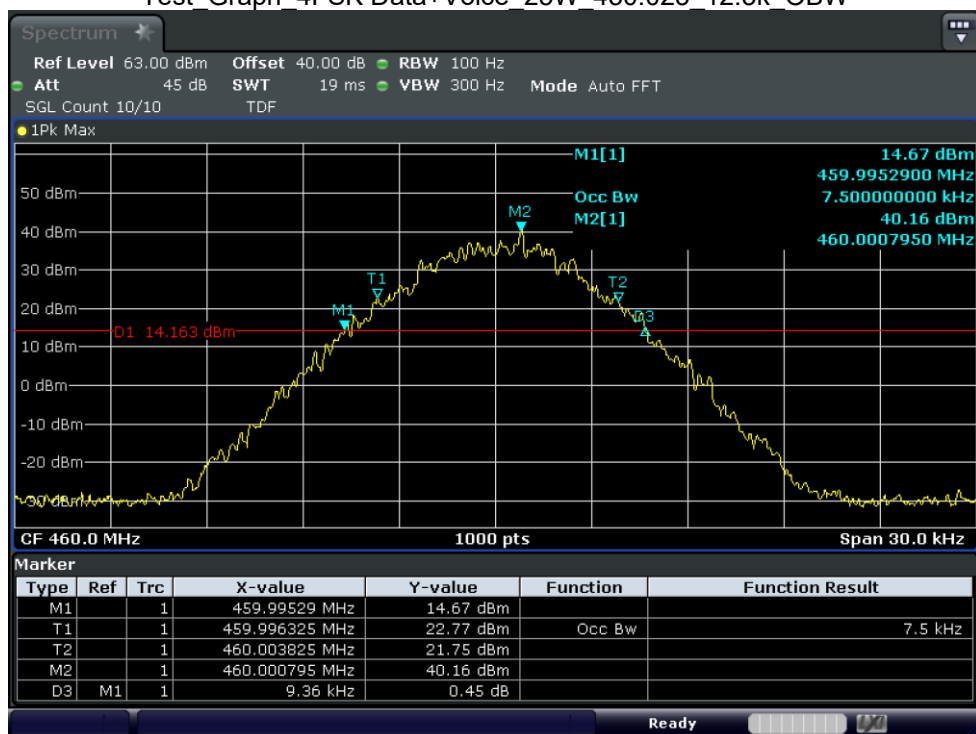
Test_Graph_4FSK Data+Voice_25W_460_12.5k_OBW
