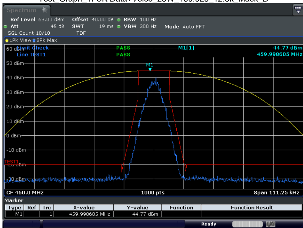
Test_Graph_4FSK Data+Voice_25W_460_12.5k_Mask_D
