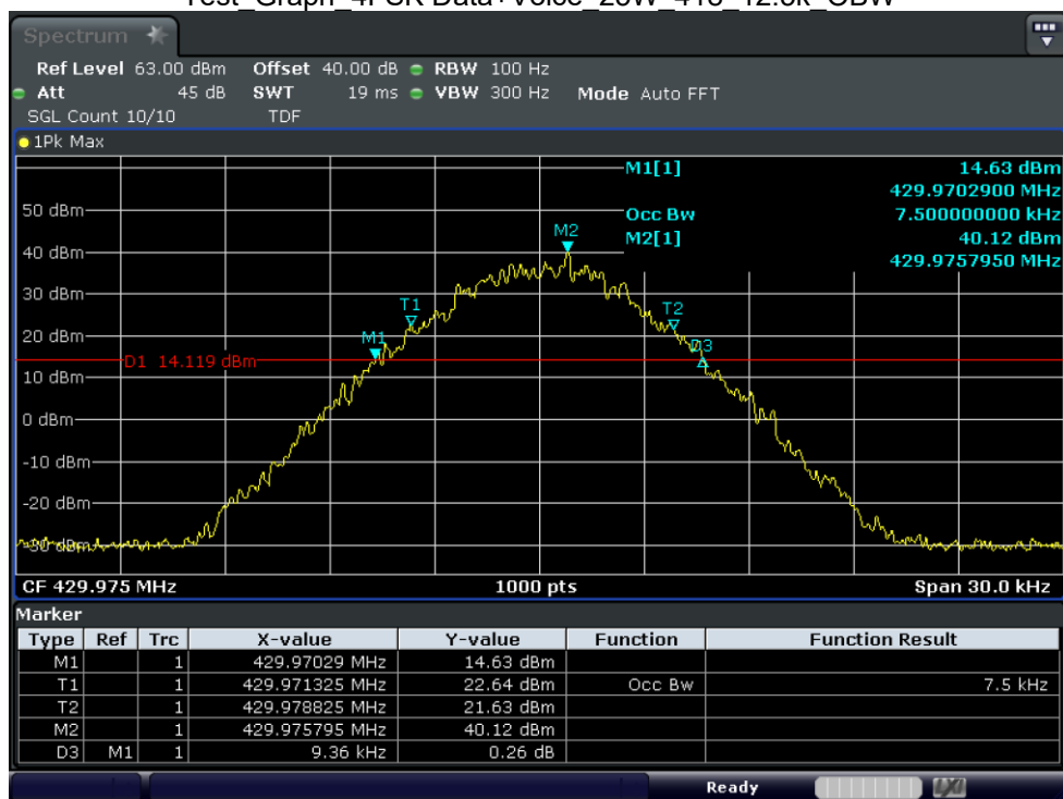
Test_Graph_4FSK Data+Voice_25W_429.975_12.5k_OBW
