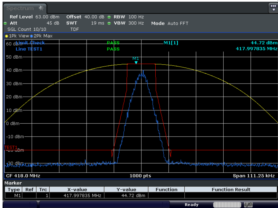
Test Graph 4FSK Data+Voice 25W 418 12.5k Mask D
