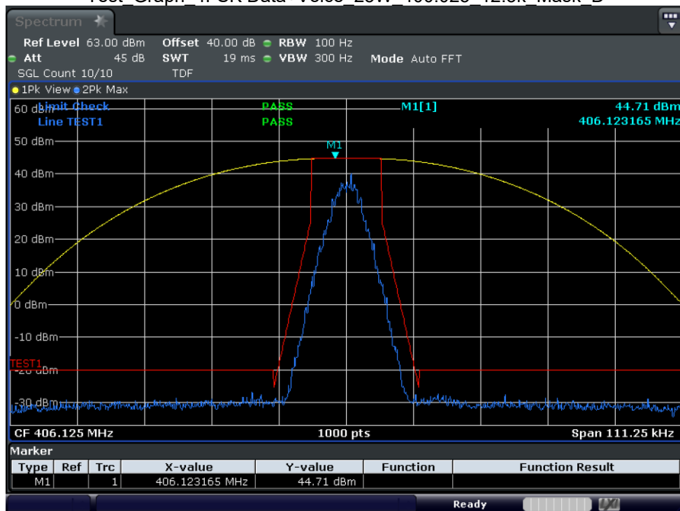
Test_Graph_4FSK Data+Voice_25W_406.125_12.5k_Mask_D
