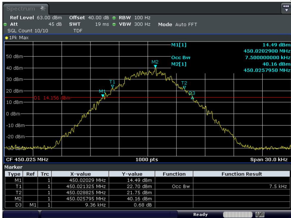
Test Graph 4FSK Data+Voice 25W 450.025 12.5k OBW
