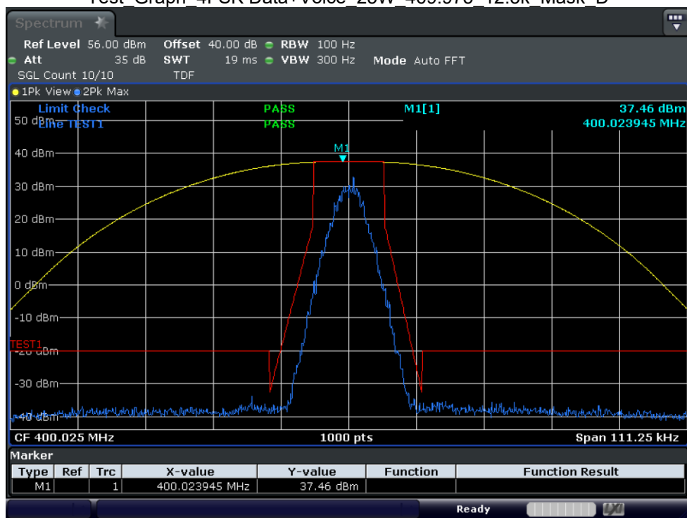
Test_Graph_4FSK Data+Voice_5W_400.025_12.5k_Mask_D
