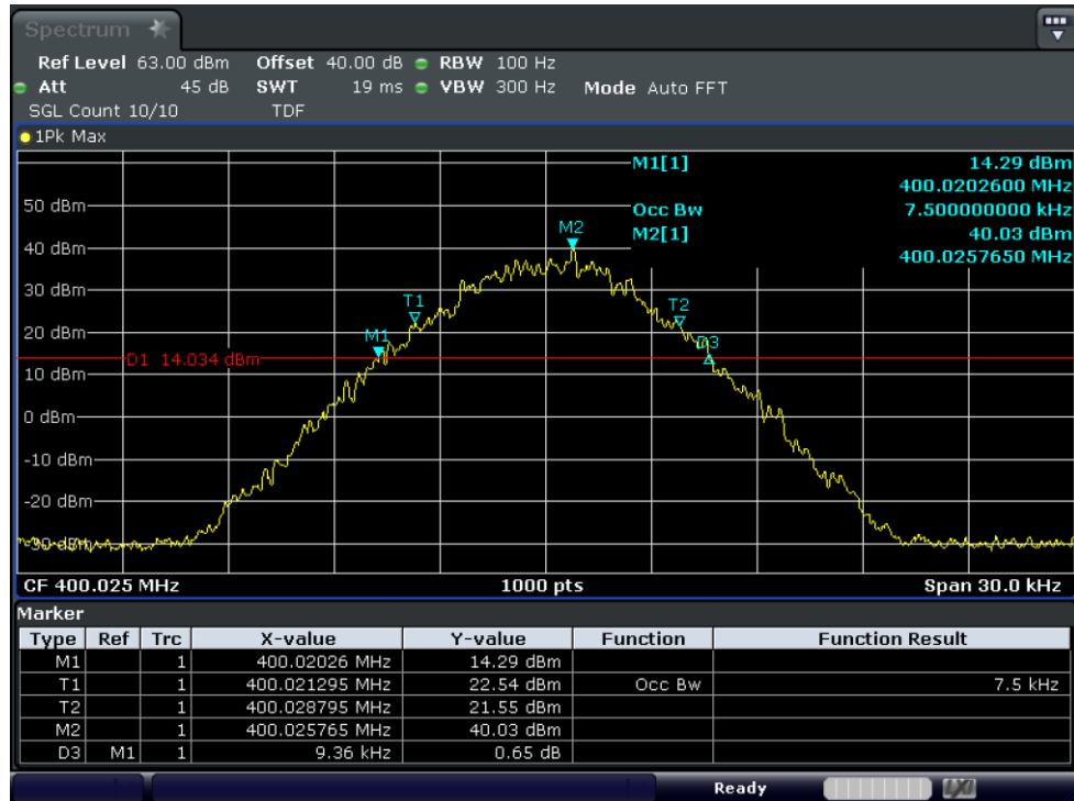
Test Graph 4FSK Data 25W 400.025 12.5k OBW
