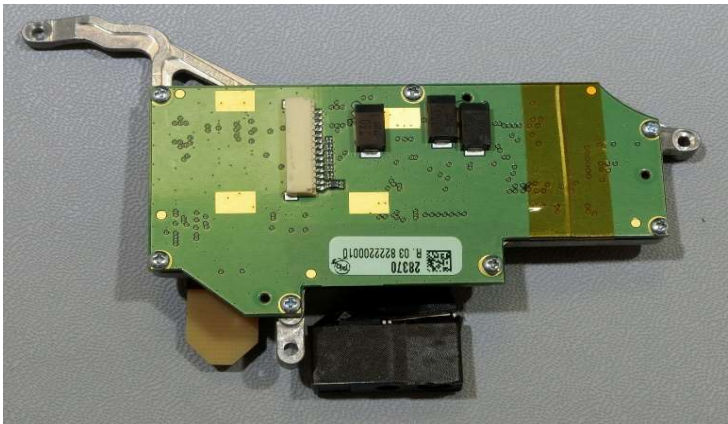
Expansion PCB with mounting bracket
