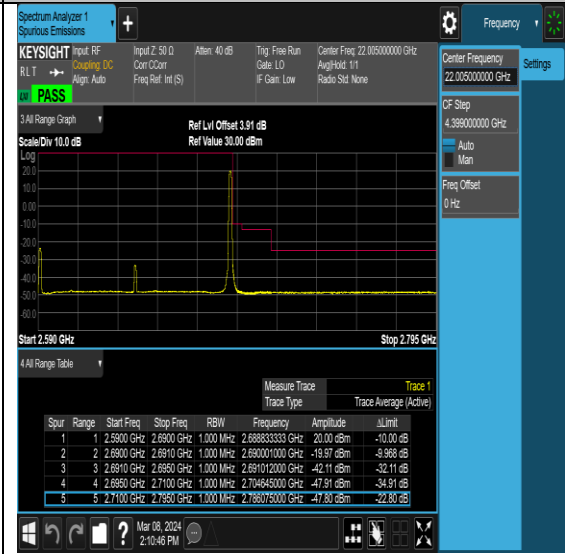
NTNV-N41-PC2-30-100-H-DFT-QPSK-Edge_1RB_Right-Ant0-PASS
