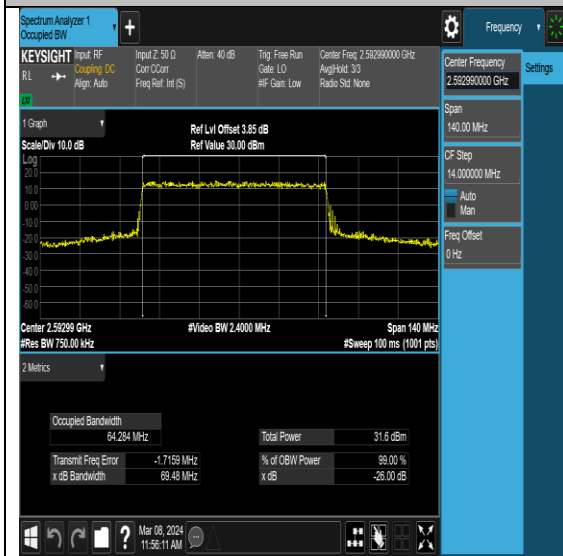
NTNV-N41-PC2-30-70-M-DFT-QPSK-Outer_Full-Ant0-PASS
