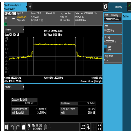
NTNV-N41-PC2-30-40-M-DFT-64QAM-Outer_Full-Ant0-PASS
