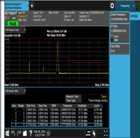
NTNV-N41-PC2-30-60-H-DFT-QPSK-Edge_1RB_Right-Ant0-PASS
