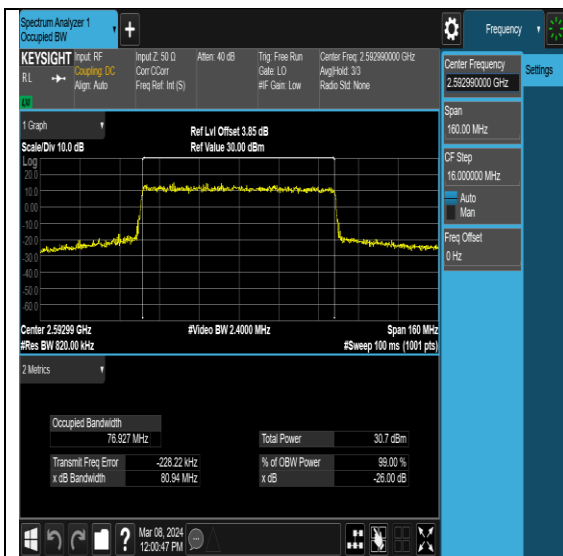
NTNV-N41-PC2-30-80-M-DFT-16QAM-Outer_Full-Ant0-PASS
