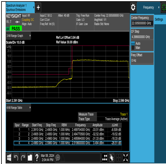
NTNV-N41-PC2-30-100-L-DFT-QPSK-Outer_Full-Ant0-PASS
