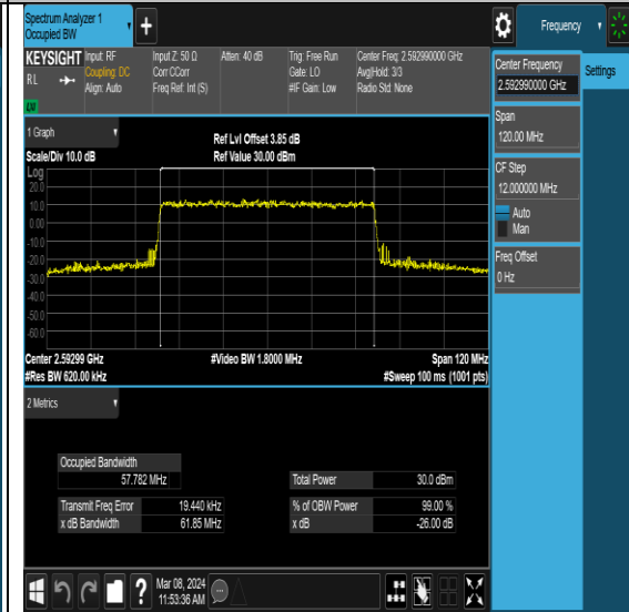
NTNV-N41-PC2-30-60-M-DFT-64QAM-Outer_Full-Ant0-PASS
