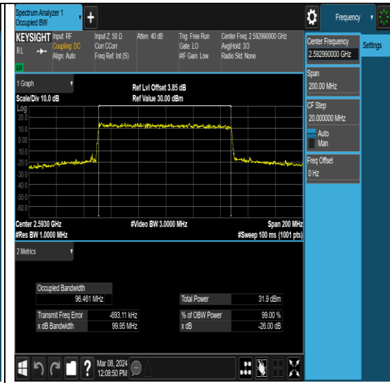
NTNV-N41-PC2-30-100-M-DFT-QPSK-Outer_Full-Ant0-PASS
