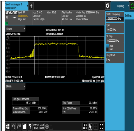
NTVN-N41-PC2-30-50-M-DFT-16QAM-Outer_Full-Ant0-PASS
