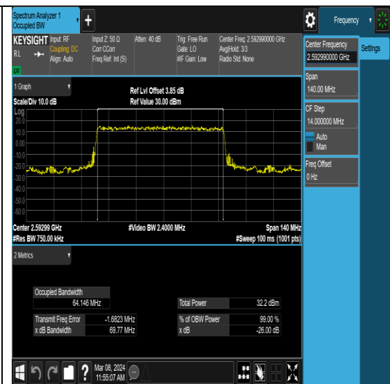
NTNV-N41-PC2-30-70-M-DFT-PI2BPSK-Outer_Full-Ant0-PASS
