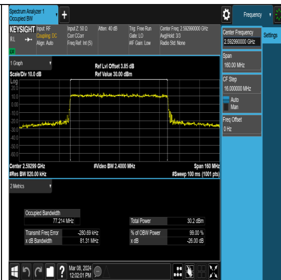
NTNV-N41-PC2-30-80-M-DFT-64QAM-Outer_Full-Ant0-PASS
