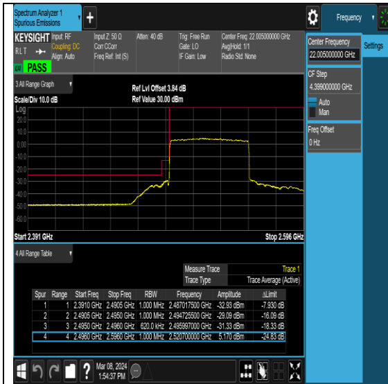
NTNV-N41-PC2-30-60-L-DFT-QPSK-Outer_Full-Ant0-PASS
