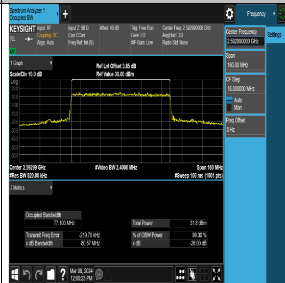
NTNV-N41-PC2-30-80-M-DFT-QPSK-Outer_Full-Ant0-PASS
