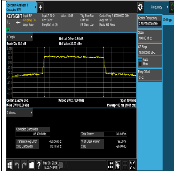
NTVN-N41-PC2-30-90-M-DFT-64QAM-Outer_Full-Ant0-PASS
