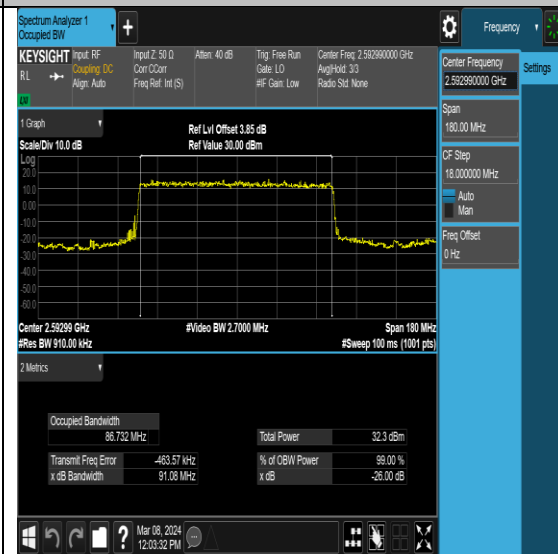
NTNV-N41-PC2-30-90-M-DFT-PI2BPSK-Outer_Full-Ant0-PASS
