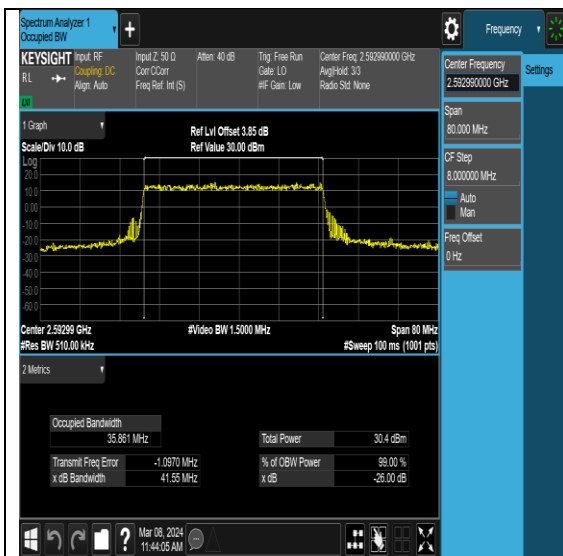
NTNV-N41-PC2-30-40-M-DFT-16QAM-Outer_Full-Ant0-PASS
