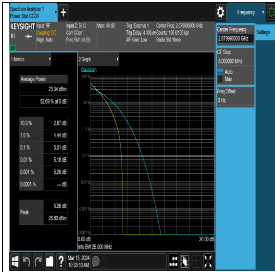
NTNV-N41-PC2-30-20-H-DFT-QPSK-Outer_Full-PASS
