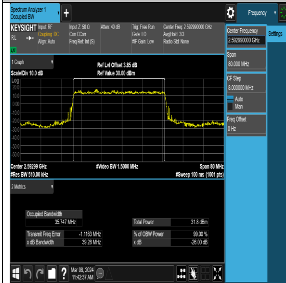
NTNV-N41-PC2-30-40-M-DFT-PI2BPSK-Outer_Full-Ant0-PASS
