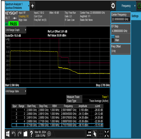
NTNV-N41-PC2-30-100-H-DFT-QPSK-Outer_Full-Ant0-PASS
