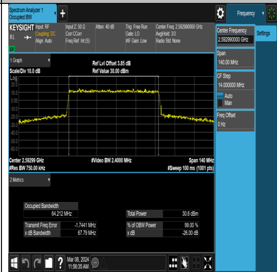
NTNV-N41-PC2-30-70-M-DFT-16QAM-Outer_Full-Ant0-PASS
