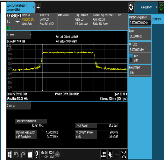
NTNV-N41-PC2-30-40-M-DFT-QPSK-Outer_Full-Ant0-PASS
