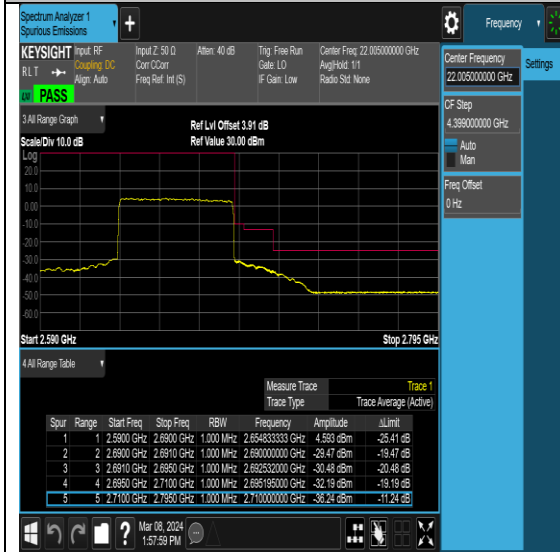
NTNV-N41-PC2-30-60-H-DFT-QPSK-Outer_Full-Ant0-PASS
