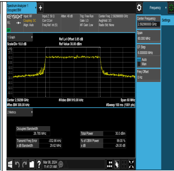
NTNV-N41-PC2-30-30-M-DFT-256QAM-Outer_Full-Ant0-PASS
