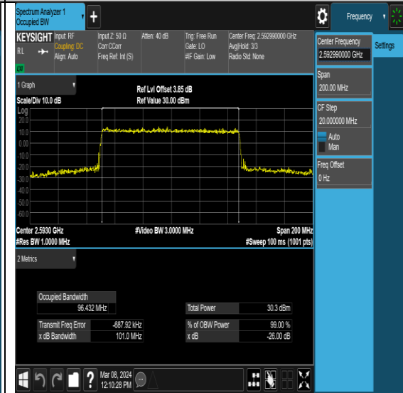
NTNV-N41-PC2-30-100-M-DFT-64QAM-Outer_Full-Ant0-PASS
