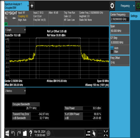
NTNV-N41-PC2-30-30-M-DFT-16QAM-Outer_Full-Ant0-PASS
