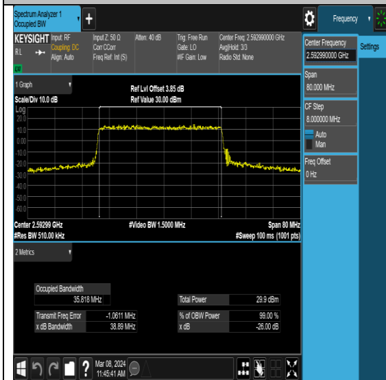
NTNV-N41-PC2-30-40-M-DFT-256QAM-Outer_Full-Ant0-PASS
