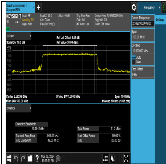
NTVN-N41-PC2-30-50-M-DFT-QPSK-Outer_Full-Ant0-PASS
