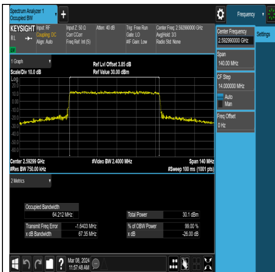
NTNV-N41-PC2-30-70-M-DFT-64QAM-Outer_Full-Ant0-PASS
