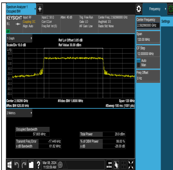
NTNV-N41-PC2-30-60-M-DFT-256QAM-Outer_Full-Ant0-PASS
