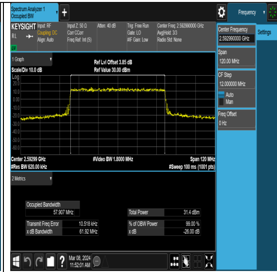
NTNV-N41-PC2-30-60-M-DFT-QPSK-Outer_Full-Ant0-PASS
