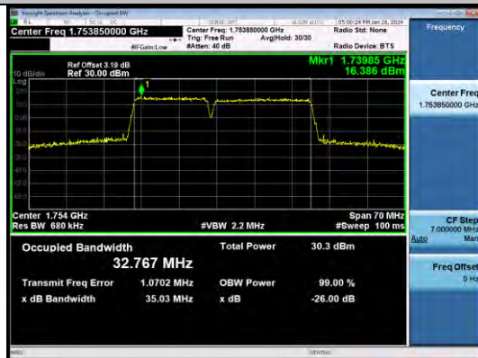
66-66-15MHz-20MHz-16QAM-16QAM-132325-132496-7 5RB#0-100RB#0-PASS
