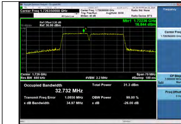
66-66-15MHz-20MHz-QPSK-QPSK-132050-132221-75R B#0-100RB#0-PASS
