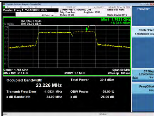
66-66-15MHz-10MHz-16QAM-16QAM-132373-132493-7 5RB#0-50RB#0-PASS
