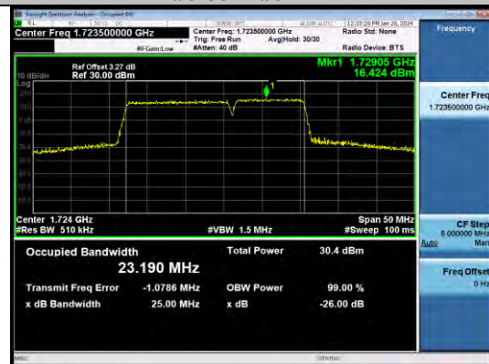
66-66-15MHz-10MHz-16QAM-16QAM-132047-132167-7 5RB#0-50RB#0-PASS
