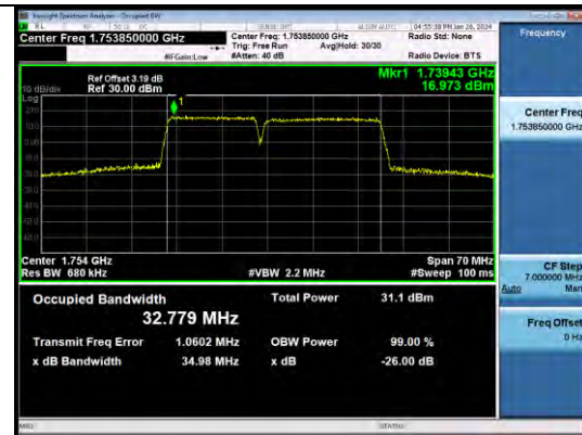
66-66-15MHz-20MHz-QPSK-QPSK-132325-132496-75R B#0-100RB#0-PASS
