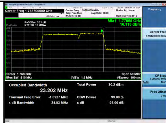
66-66-15MHz-10MHz-16QAM-16QAM-132499-132619-7 5RB#0-50RB#0-PASS
