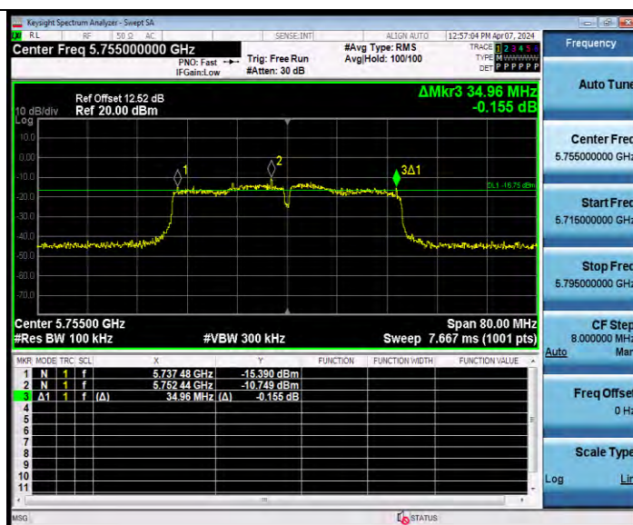
11N40MIMO Ant8 5755
