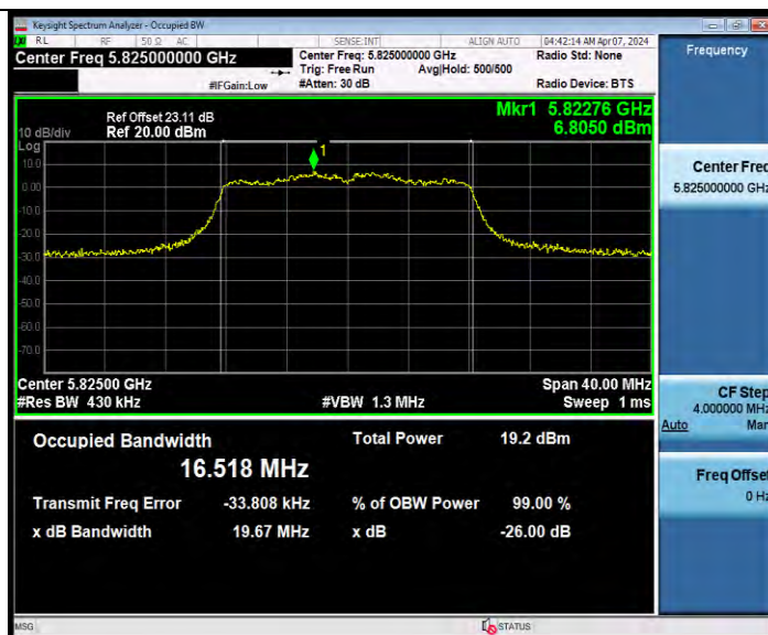
11A-CDD Ant8 5825
