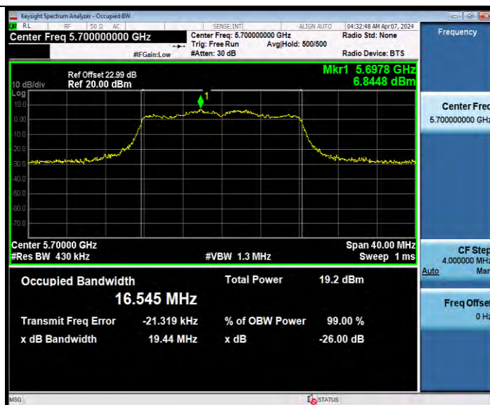
11A-CDD Ant8 5700
