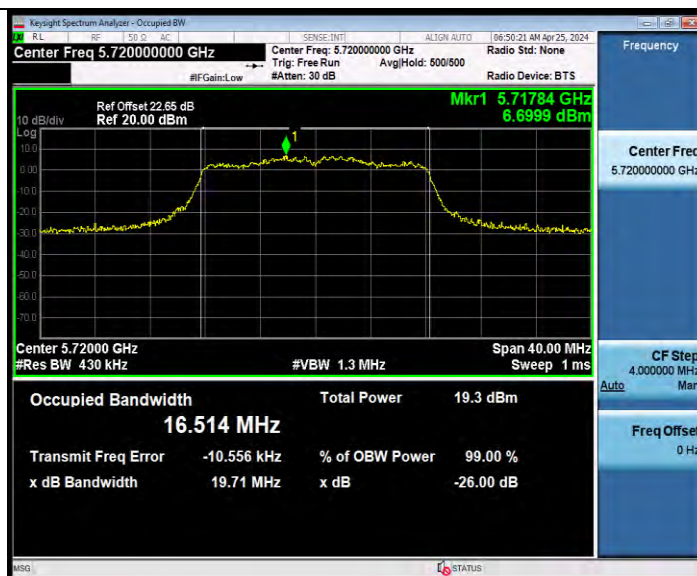
11A-CDD Ant8 5720
