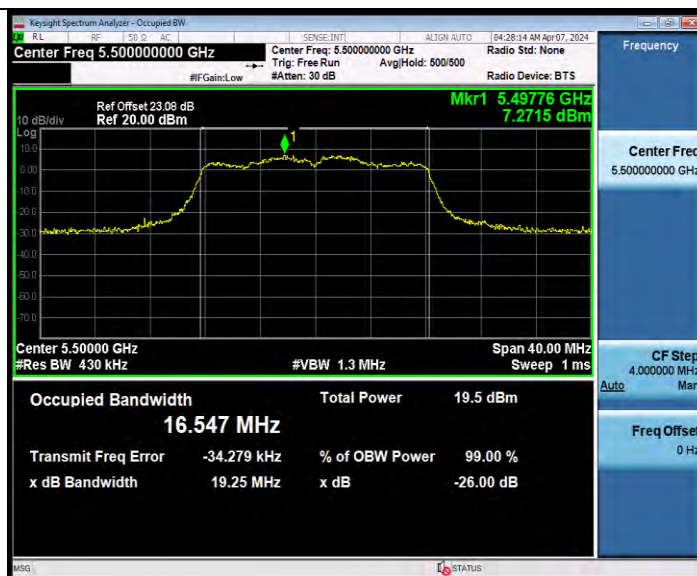
11A-CDD Ant8 5500
