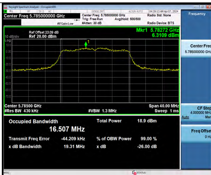
11A-CDD Ant8 5785
