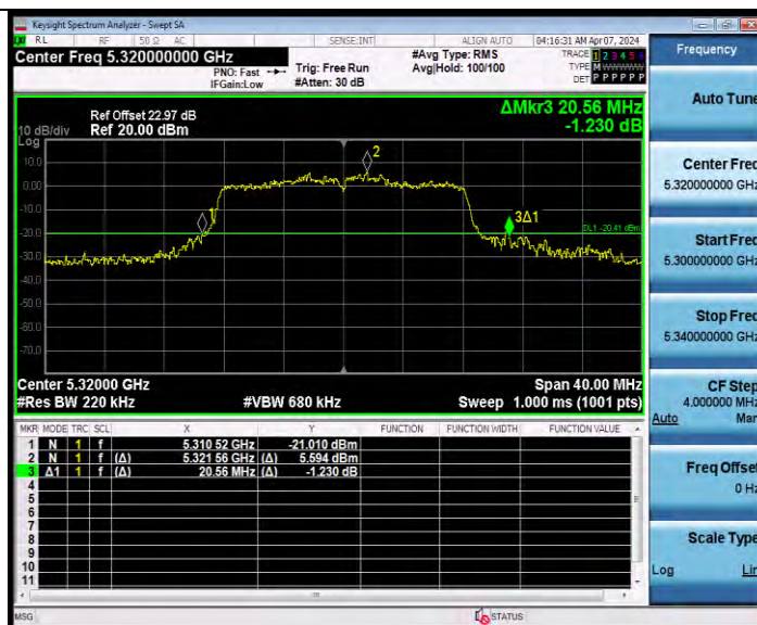
11A-CDD Ant8 5320
