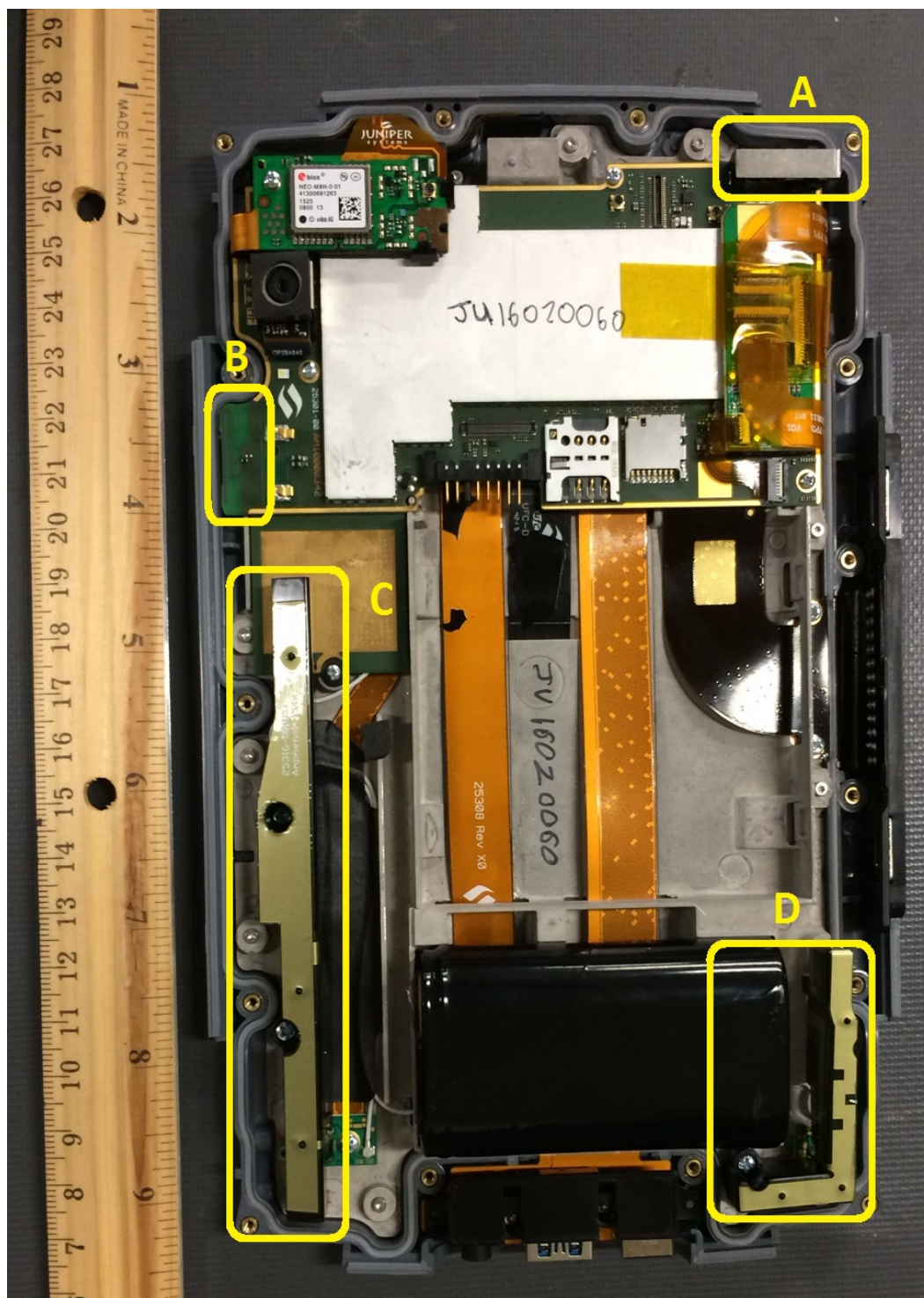
Figure 4: Assembled - View 2
