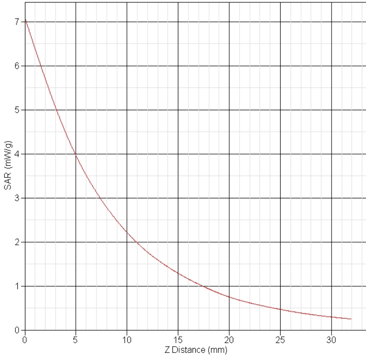
SAR-Z Axis at Hotspot x:0.25 y:-0.15
