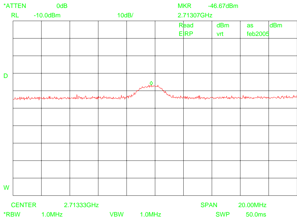
Plot 19 – Emission in the restriced band 2.69 – 2.90 GHz, -21.2 dBm corresponds to 74 dBμV/m (Continuous transmit mode on channel 1, measurement results in peak mode)
