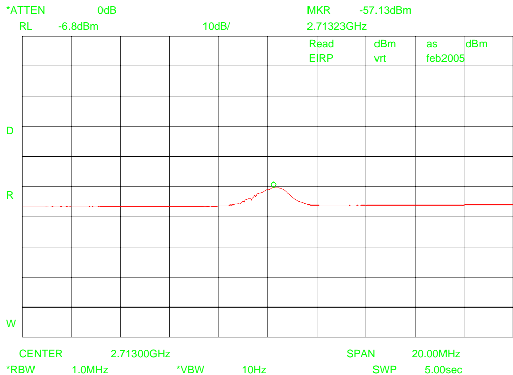
Plot 20 – Emission in the restriced band 2.69 – 2.90 GHz, -41.2 dBm corresponds to 54 dBµV/m (Continuous transmit mode on channel 1, offset of 10log(21ms/100ms) for peak/average ratio, measurement results in average mode)
