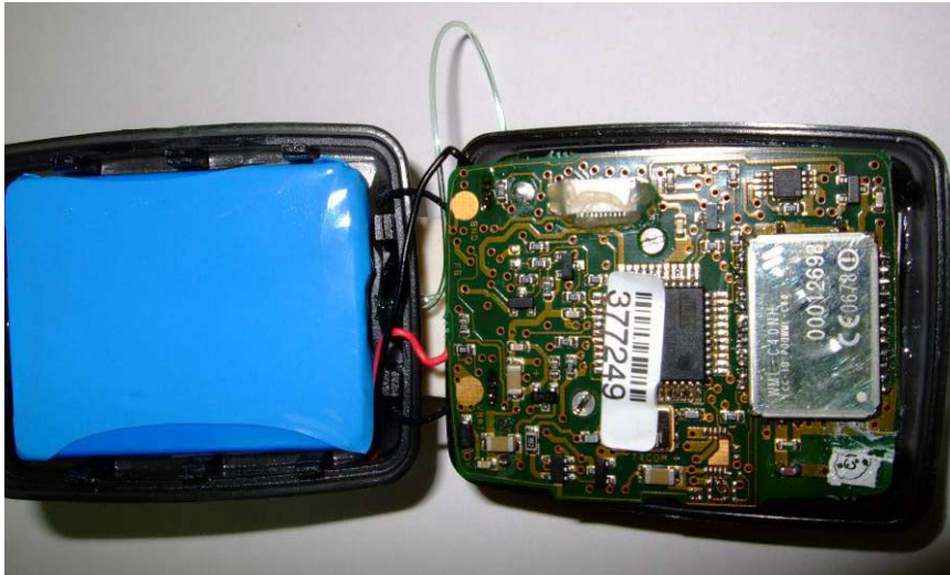
ASSEMBLY VIEW :
