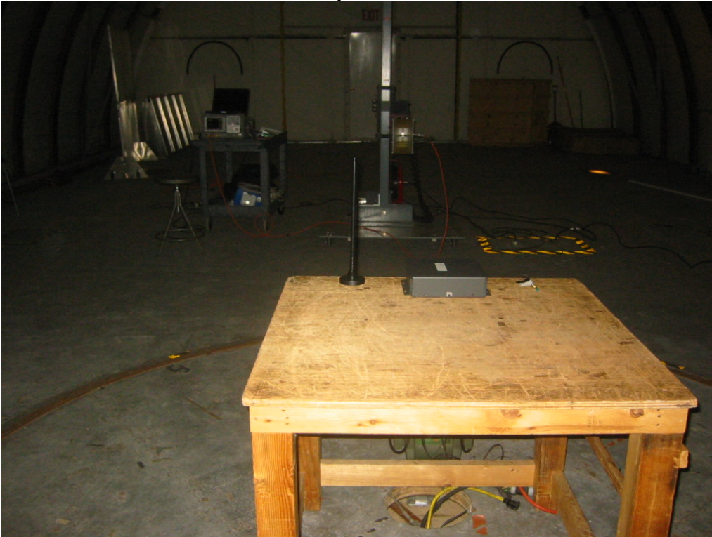
1-2 GHz Radiated Emission
