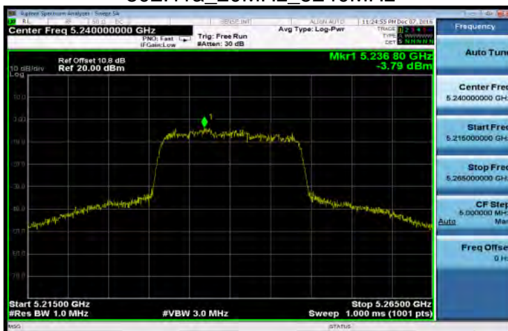
802.11a_20MHz_5240MHz
