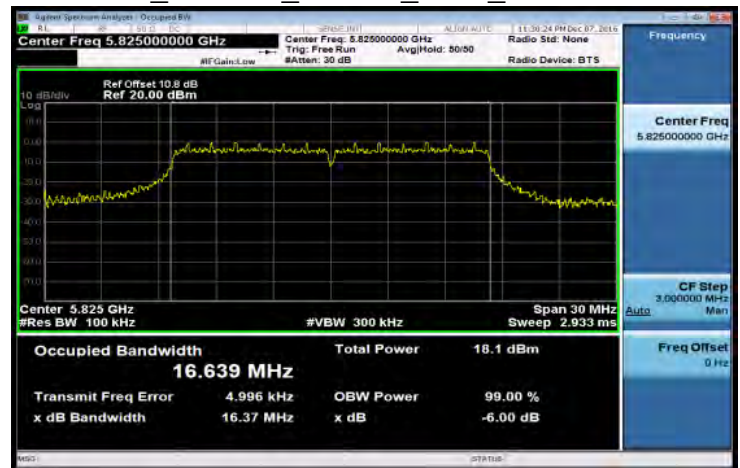
FCC_802.11a_20MHz_Main_5825MHz
