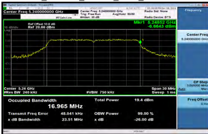
FCC_802.11a_20MHz_Main_5240MHz
