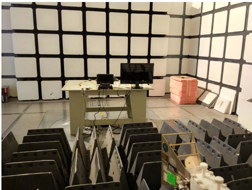
Radiated Emissions – Rear View (Above 1 GHz, With Base)
