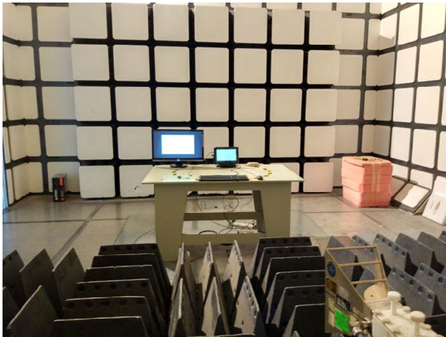
Radiated Emissions – Front View (Above 1 GHz, With Base)
