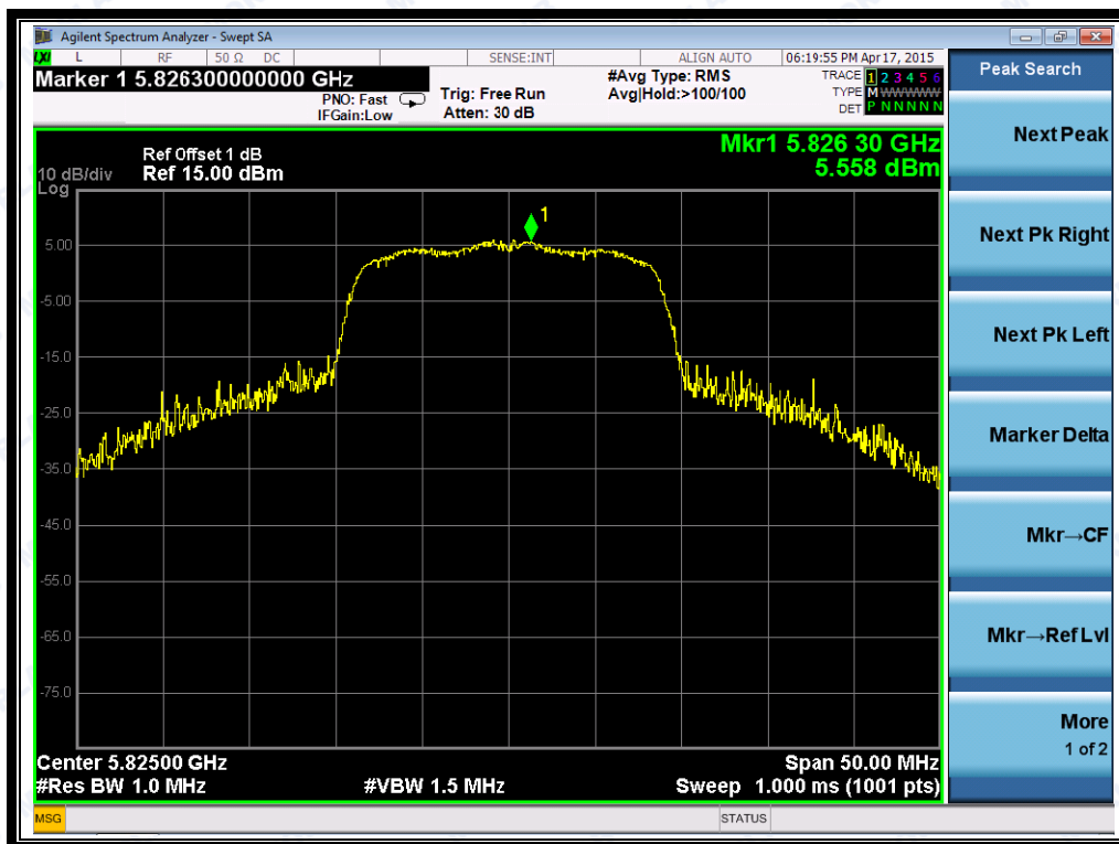
(Channel 165: 5825MHz @ 802.11n-20MHz)
