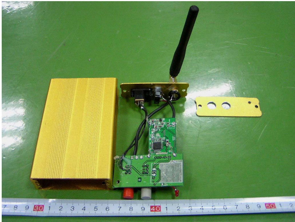
EUT – Board Assembly Top Components View
