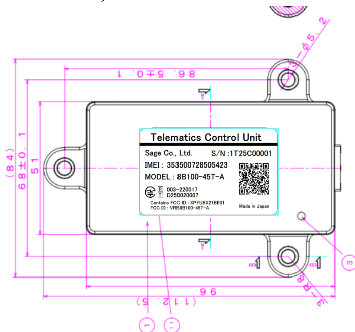
Label layout
