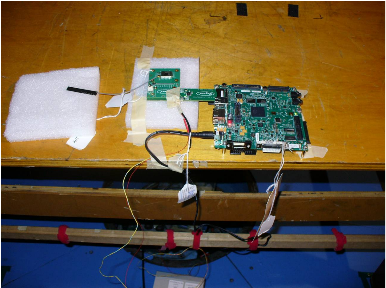
Figure 5: Radiated Emissions With PCB Antenna– Top View
