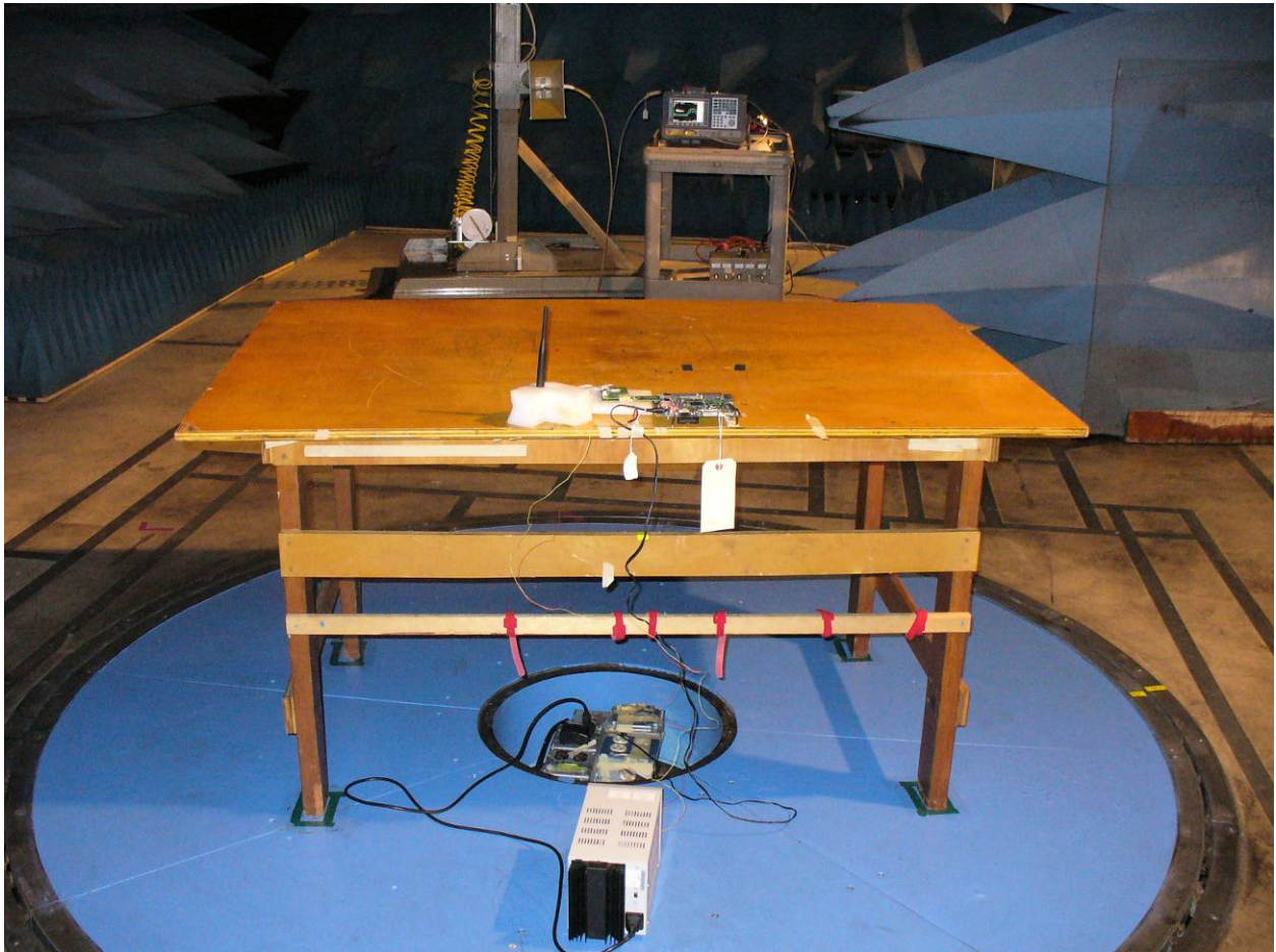
Figure 1: Radiated Emissions With Dipole Antenna– Back View
