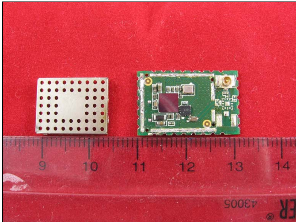
Figure 1: Internal Photo – Front – Shield Removed
