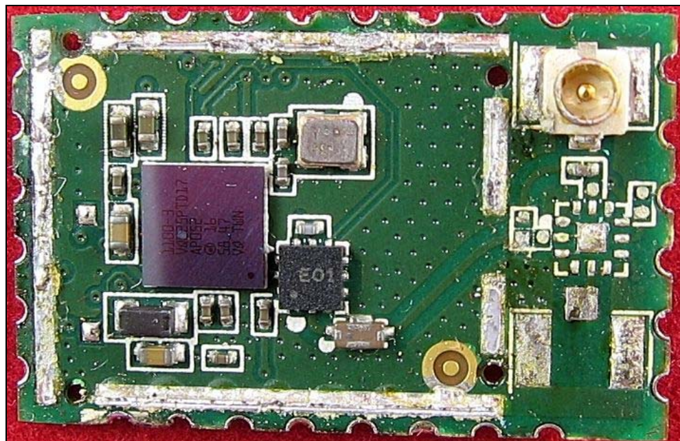
Figure 2: Internal Photo – Front – Shield Removed Close-up
