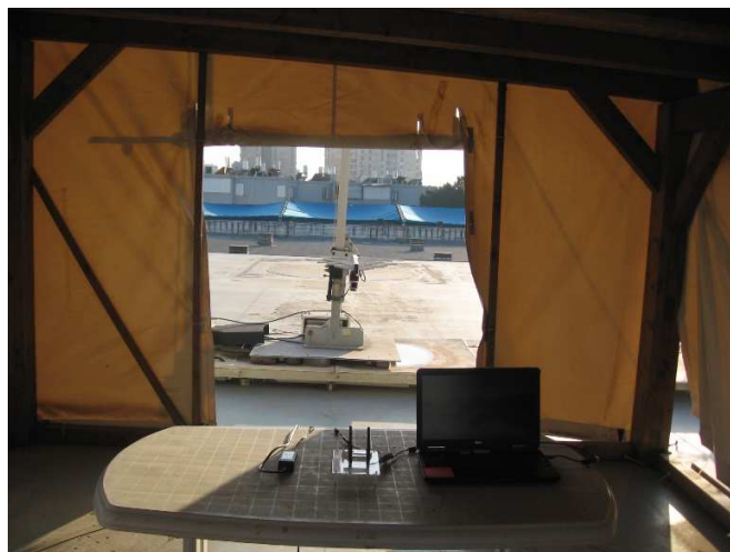
Figure 4. Radiated Emission Test, 200.0-1000.0 MHz
