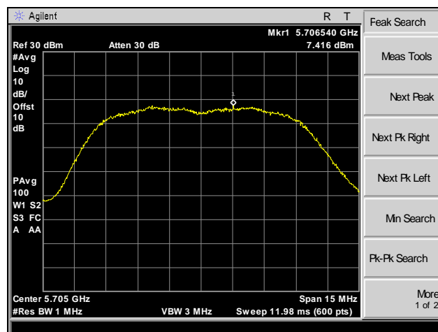
Plot 41. Maximum Power Spectral Density, 5705 MHz, 10 MHz, Channel 0
