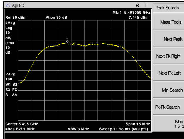
Plot 39. Maximum Power Spectral Density, 5495 MHz, 10 MHz, Channel 0
