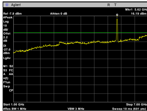
Plot 62. Radiated Spurious Emissions, 5620 MHz, 20 MHz, 1 GHz – 7 GHz
