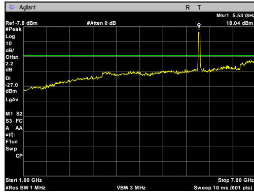
Plot 61. Radiated Spurious Emissions, 5540 MHz, 20 MHz, 1 GHz – 7 GHz
