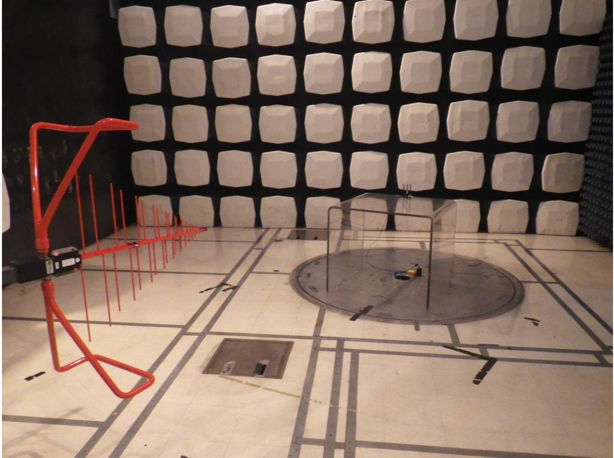
Photograph 1. Radiated Spurious Emissions, Below 1 GHz
