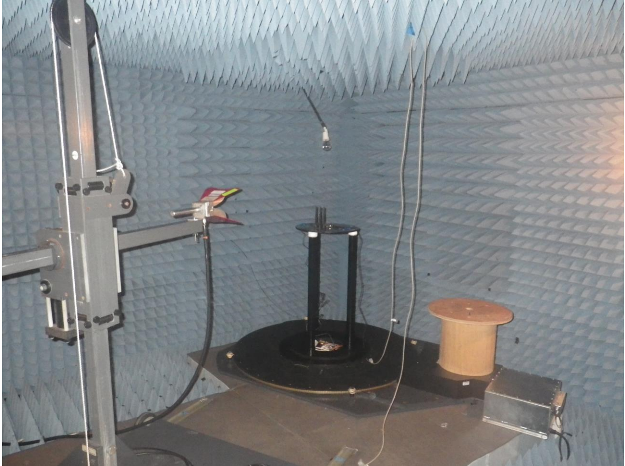
Photograph 2. Radiated Spurious Emissions, Above 1 GHz
