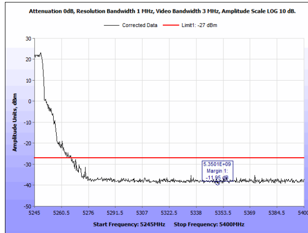
Plot 38. Radiated Band Edge, High Channel, 10 MHz, Peak
