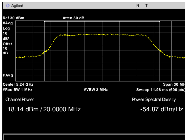
Plot 14. Output Power, High Channel, 20 MHz
