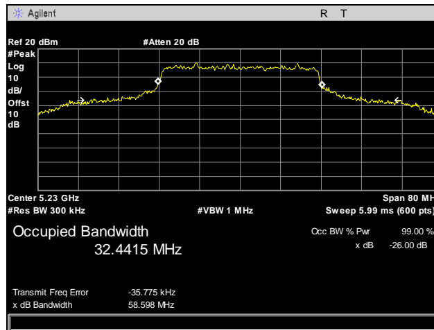
Plot 8. Occupied Bandwidth, High Channel, 40 MHz
