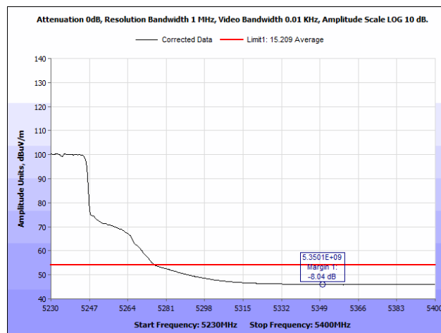
Plot 45. Radiated Band Edge, High Channel, 40 MHz, Average
