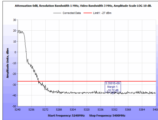
Plot 42. Radiated Band Edge, High Channel, 20 MHz, Peak
