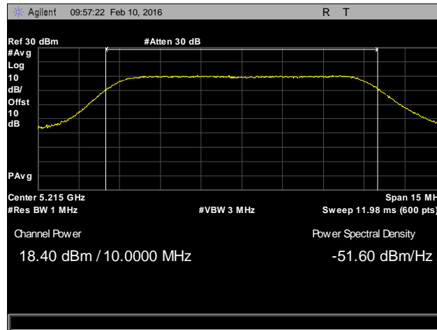
Plot 10. Output Power, Mid Channel, 10 MHz
