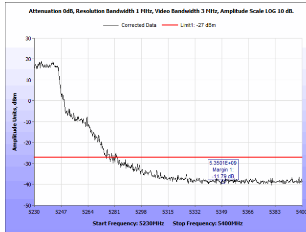
Plot 46. Radiated Band Edge, High Channel, 40 MHz, Peak
