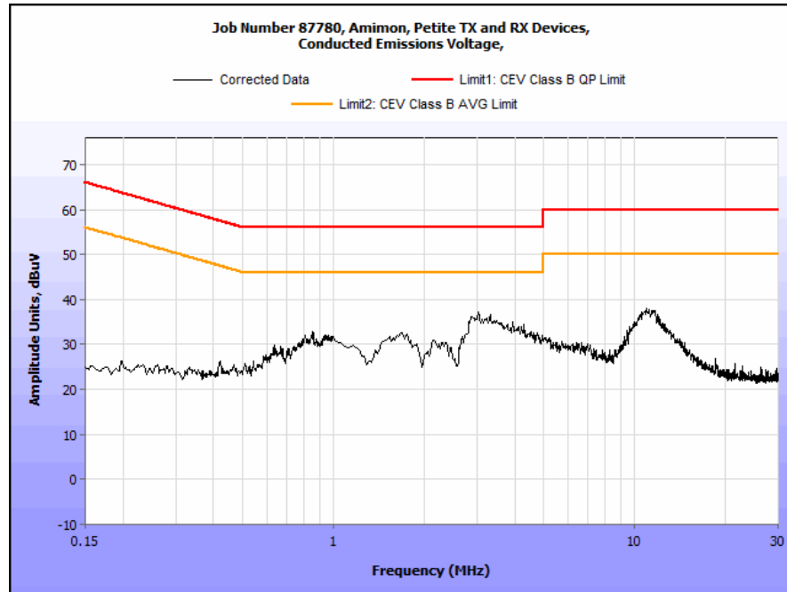
Plot 48. Conducted Emission, Neutral Line Plot
