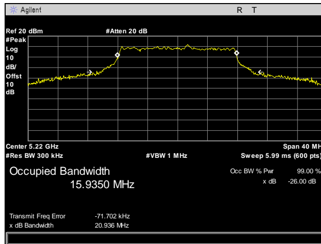
Plot 5. Occupied Bandwidth, Mid Channel, 20 MHz
