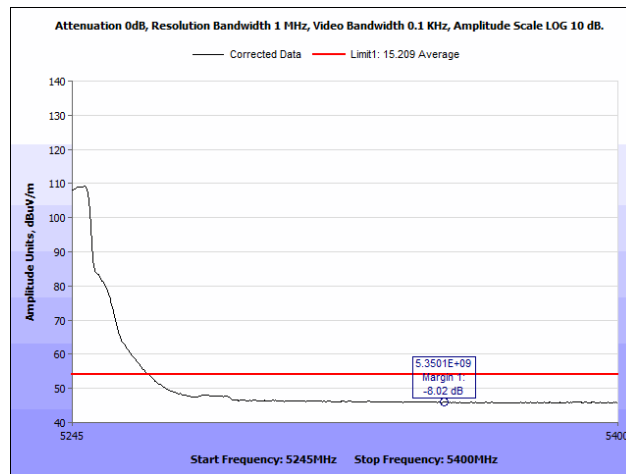
Plot 37. Radiated Band Edge, High Channel, 10 MHz, Average
