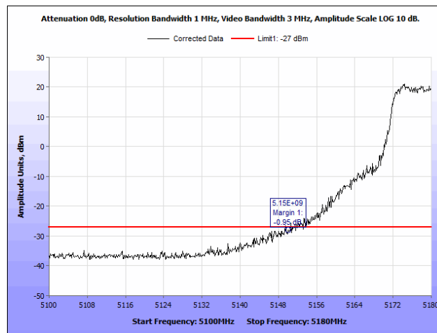
Plot 40. Radiated Band Edge, Low Channel, 20 MHz, Peak
