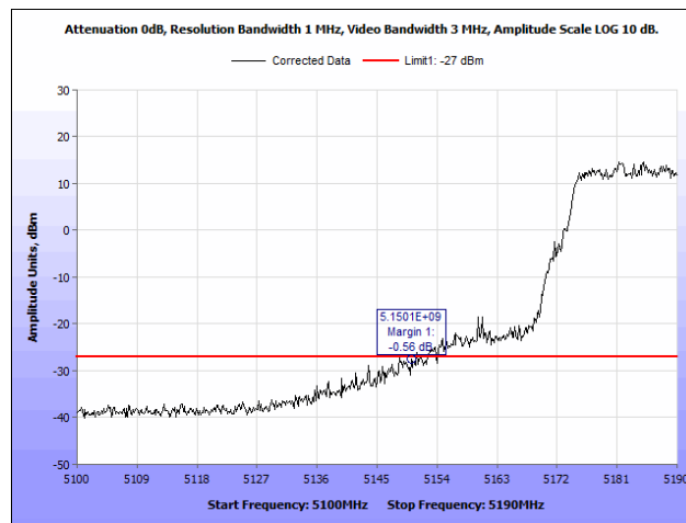
Plot 44. Radiated Band Edge, Low Channel, 40 MHz, Peak
