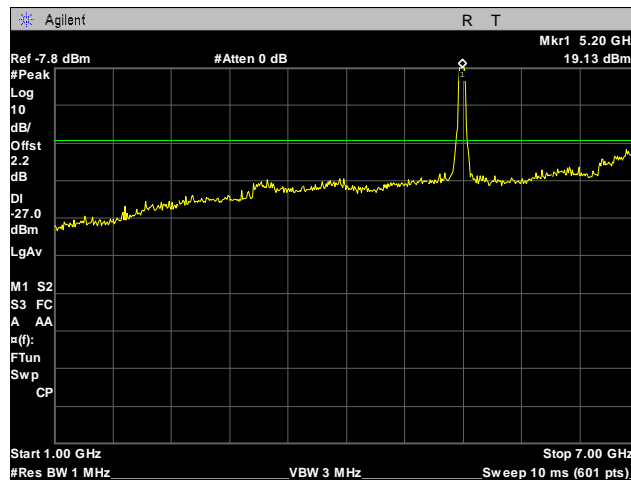
Plot 32. Radiated Spurious Emissions, Low Channel, 40 MHz, 1 GHz – 7 GHz
