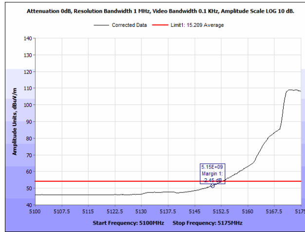
Plot 35. Radiated Band Edge, Low Channel, 10 MHz, Average
