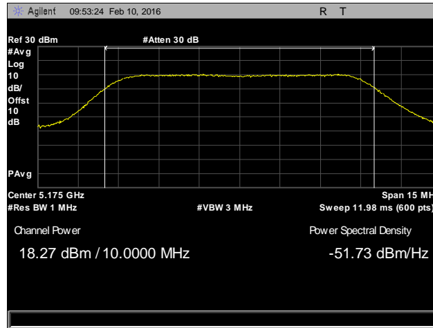
Plot 9. Output Power, Low Channel, 10 MHz
