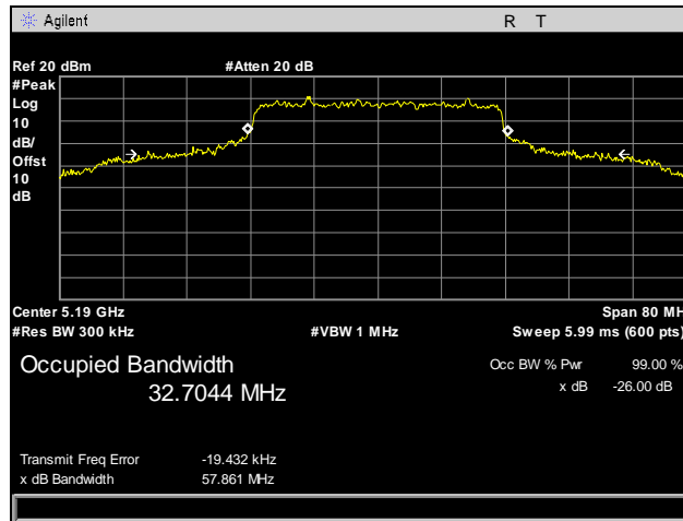
Plot 7. Occupied Bandwidth, Low Channel, 40 MHz
