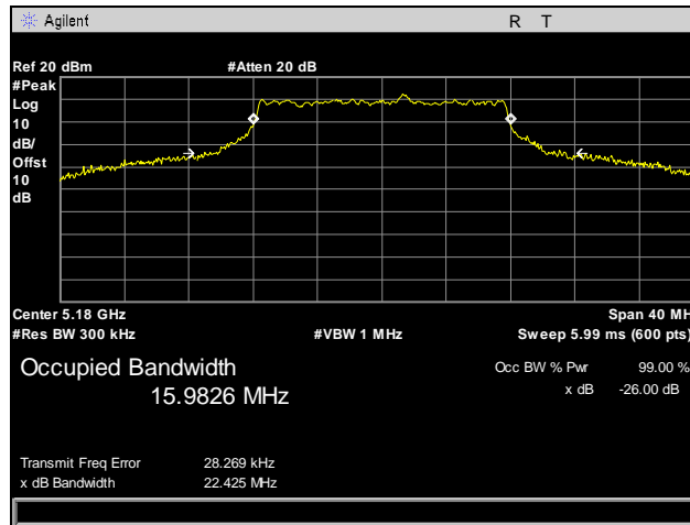
Plot 4. Occupied Bandwidth, Low Channel, 20 MHz
