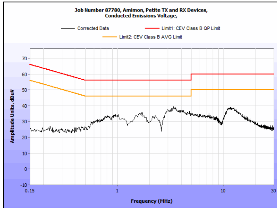
Plot 47. Conducted Emission, Phase Line Plot
