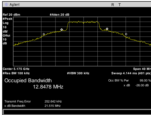
Plot 1. Occupied Bandwidth, Low Channel, 10 MHz
