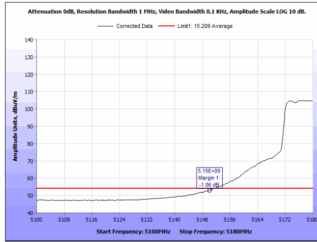
Plot 39. Radiated Band Edge, Low Channel, 20 MHz, Average
