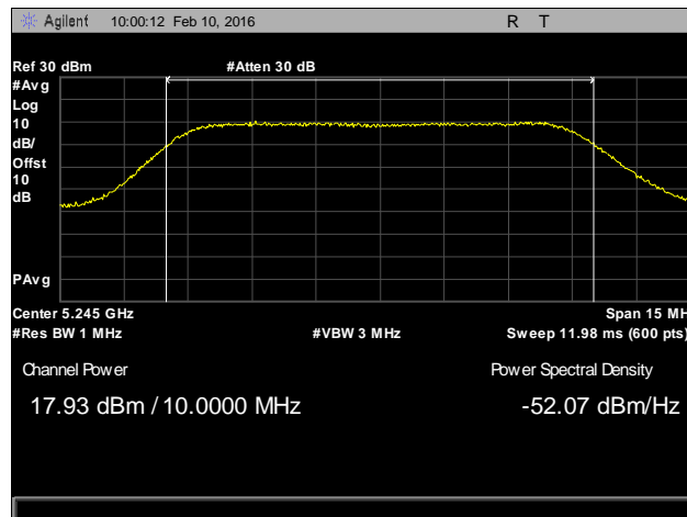
Plot 11. Output Power, High Channel, 10 MHz
