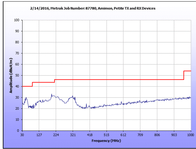
Plot 31. Radiated Spurious Emissions, Low Channel, 40 MHz, 30 MHz – 1 GHz
