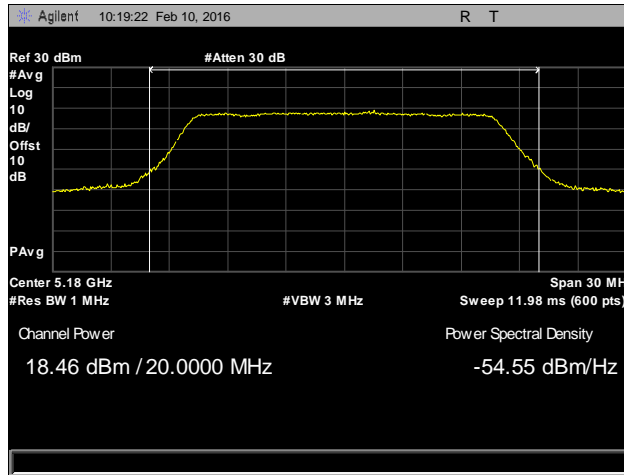
Plot 12. Output Power, Low Channel, 20 MHz
