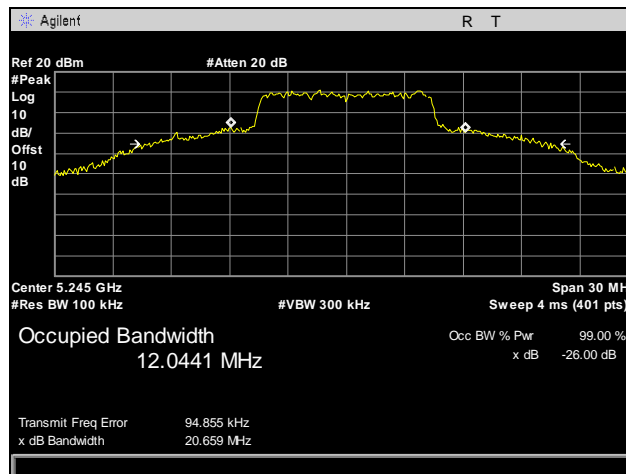
Plot 3. Occupied Bandwidth, High Channel, 10 MHz
