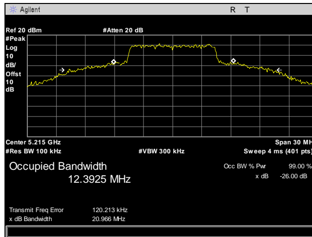
Plot 2. Occupied Bandwidth, Mid Channel, 10 MHz
