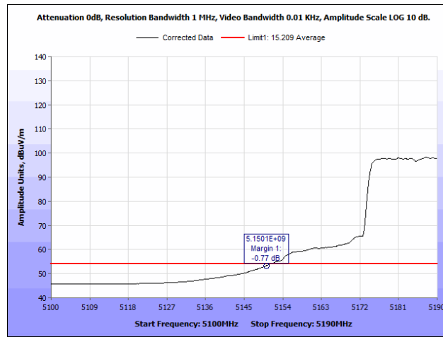
Plot 43. Radiated Band Edge, Low Channel, 40 MHz, Average
