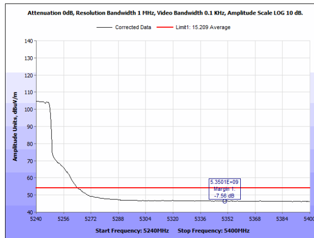
Plot 41. Radiated Band Edge, High Channel, 20 MHz, Average
