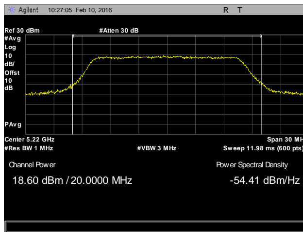
Plot 13. Output Power, Mid Channel, 20 MHz
