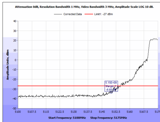
Plot 36. Radiated Band Edge, Low Channel, 10 MHz, Peak
