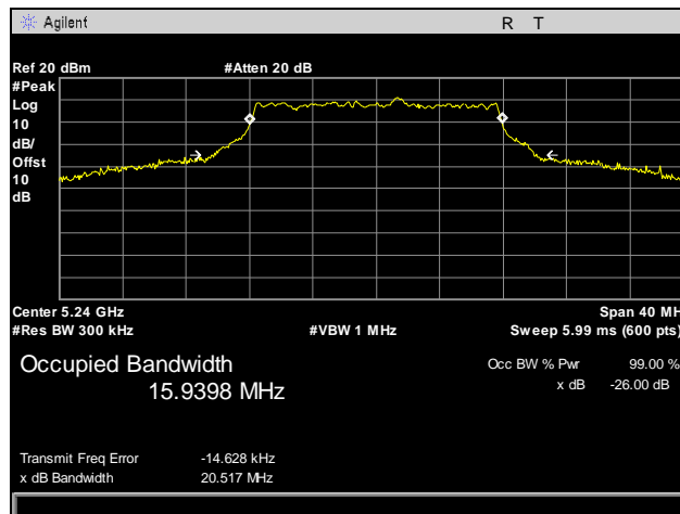
Plot 6. Occupied Bandwidth, High Channel, 20 MHz
