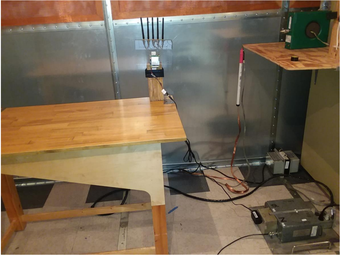
Photograph 3. Conducted Emissions, Test Setup
