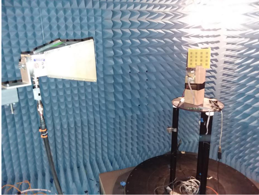
Photograph 1. Radiated Spurious above 1GHz Test Setup, 11dBi Configuration
