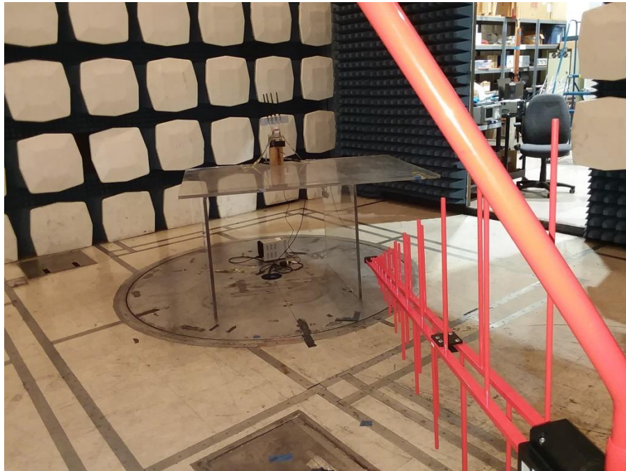
Photograph 1. Radiated Emissions, 4x4 Test Setup Below 1GHz
